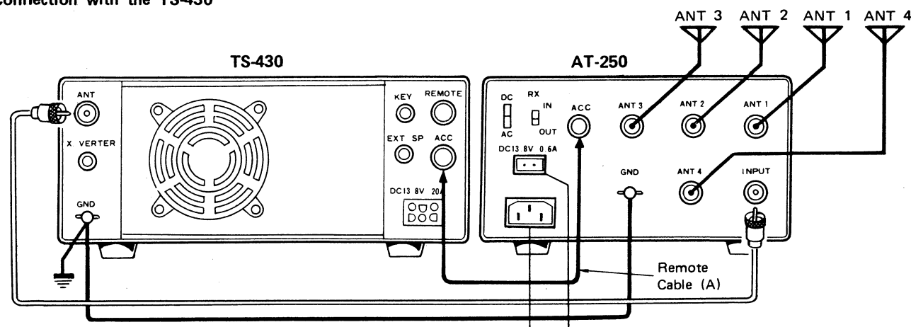
Fig. 1 To AC source To DC source
