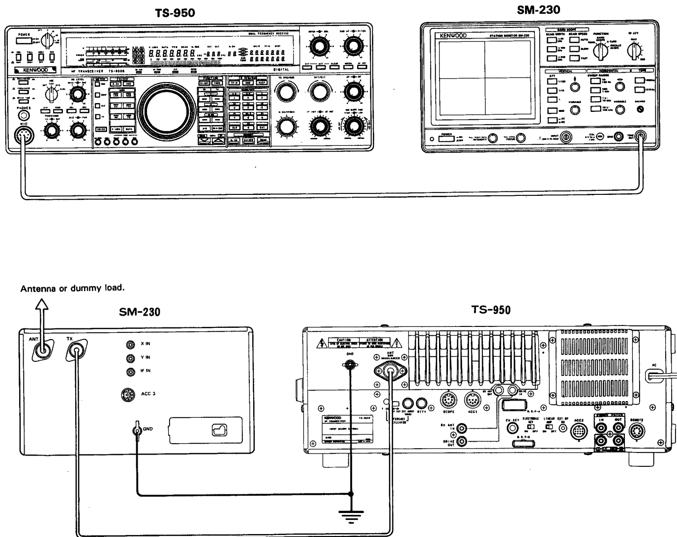
Figure 5. Hook-up of transmitting monitor
