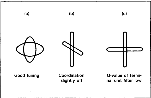
Figure 13. RTTY Cross-Pattern
