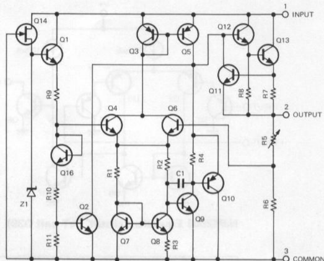
TA78L005AP Equivalent circuit (AT unit Q27)
