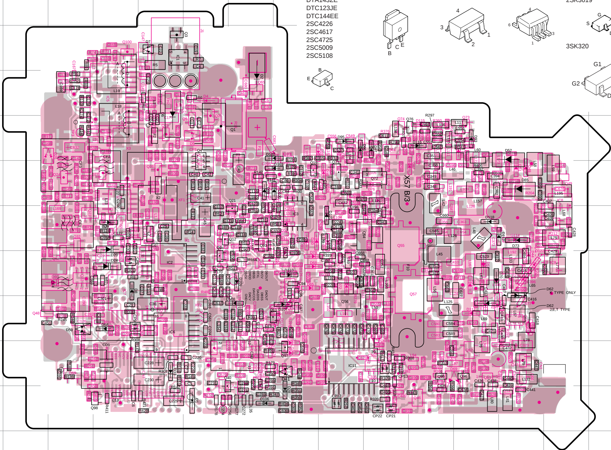
TX-RX UNIT (X57-686X-XX) (B/3) Component Side View + Foil Side View
