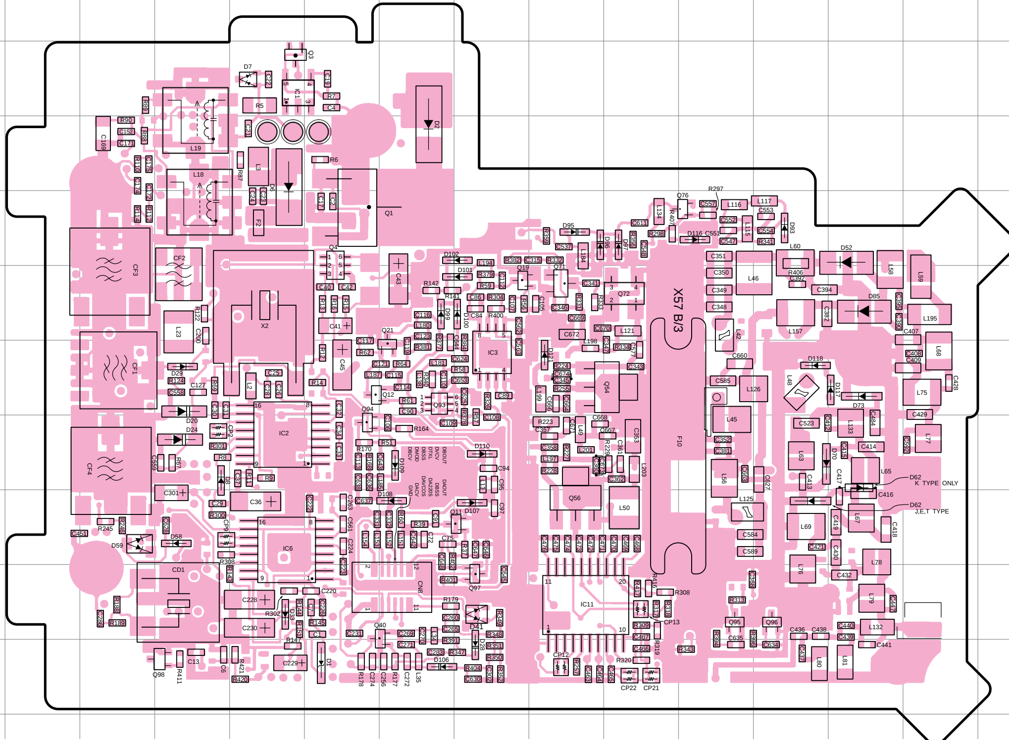
TX-RX UNIT (X57-686X-XX) (B/3) Component Side View
