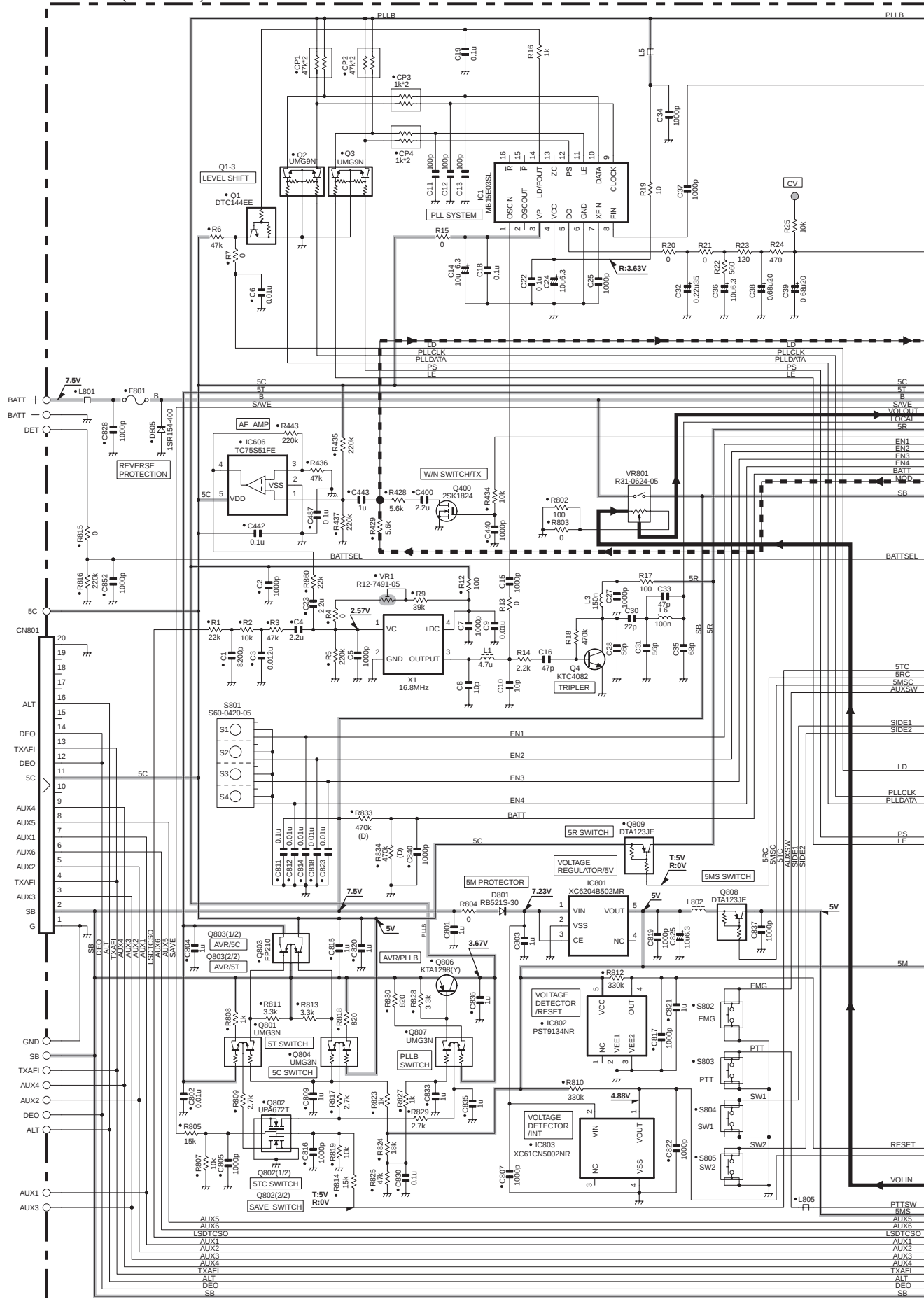
TX-RX UNIT (X57-6720-10)
