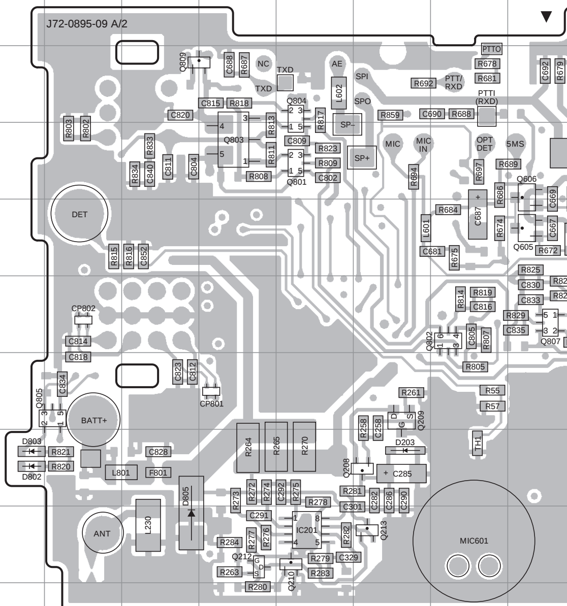
TX-RX UNIT (X57-6720-10) Component side view (J72-0895-09)
