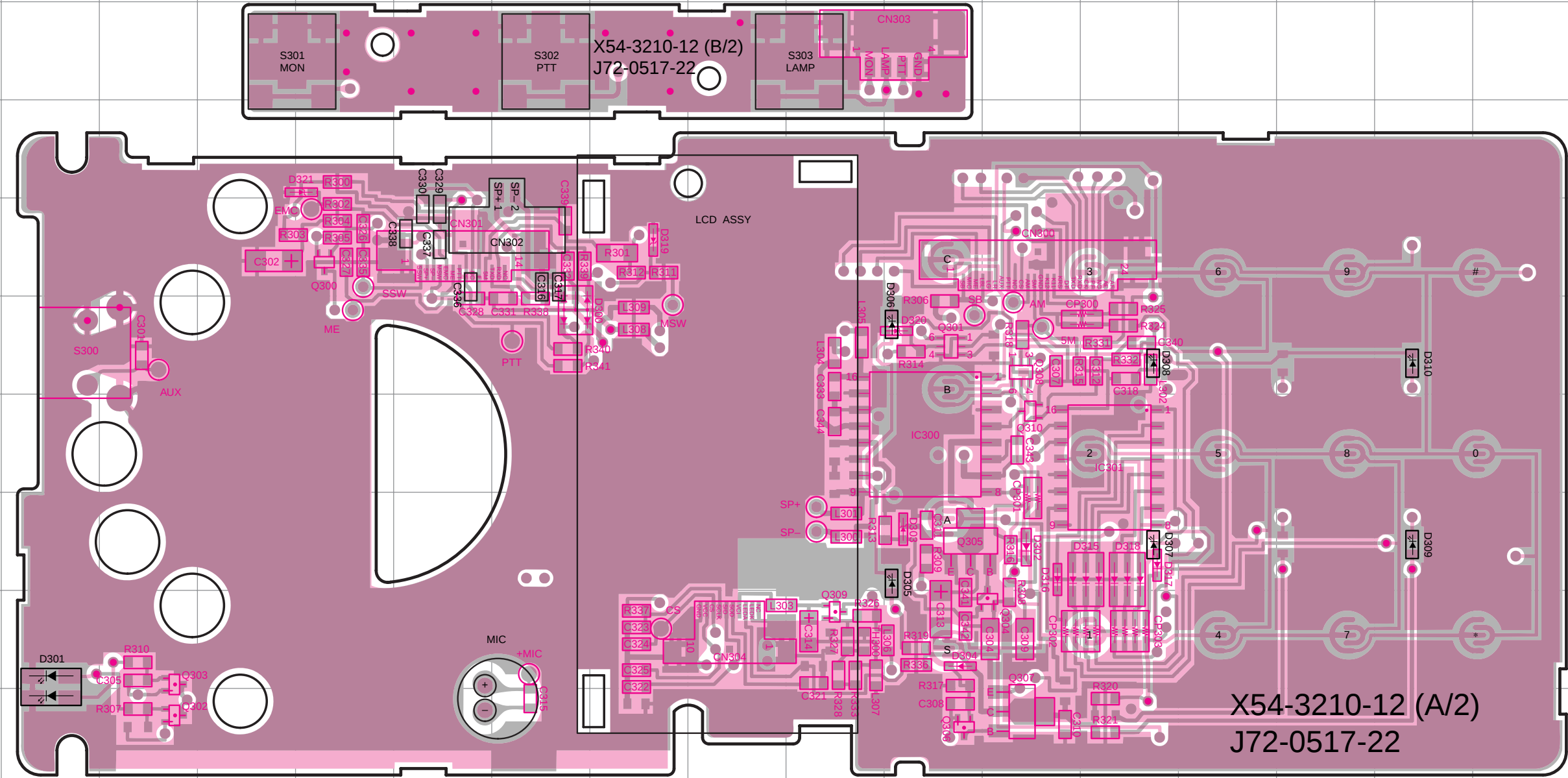
DISPLAY UNIT (X54-3210-12) Component Side + Foil Side View
