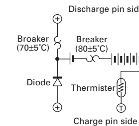
KNB-17A Circuit Diagram
