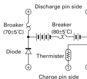
KNB-16A Circuit Diagram
