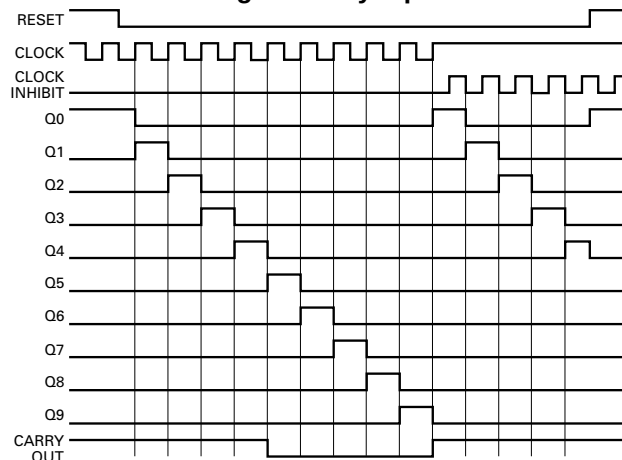
Fig. 12 Decade counter timing chart
