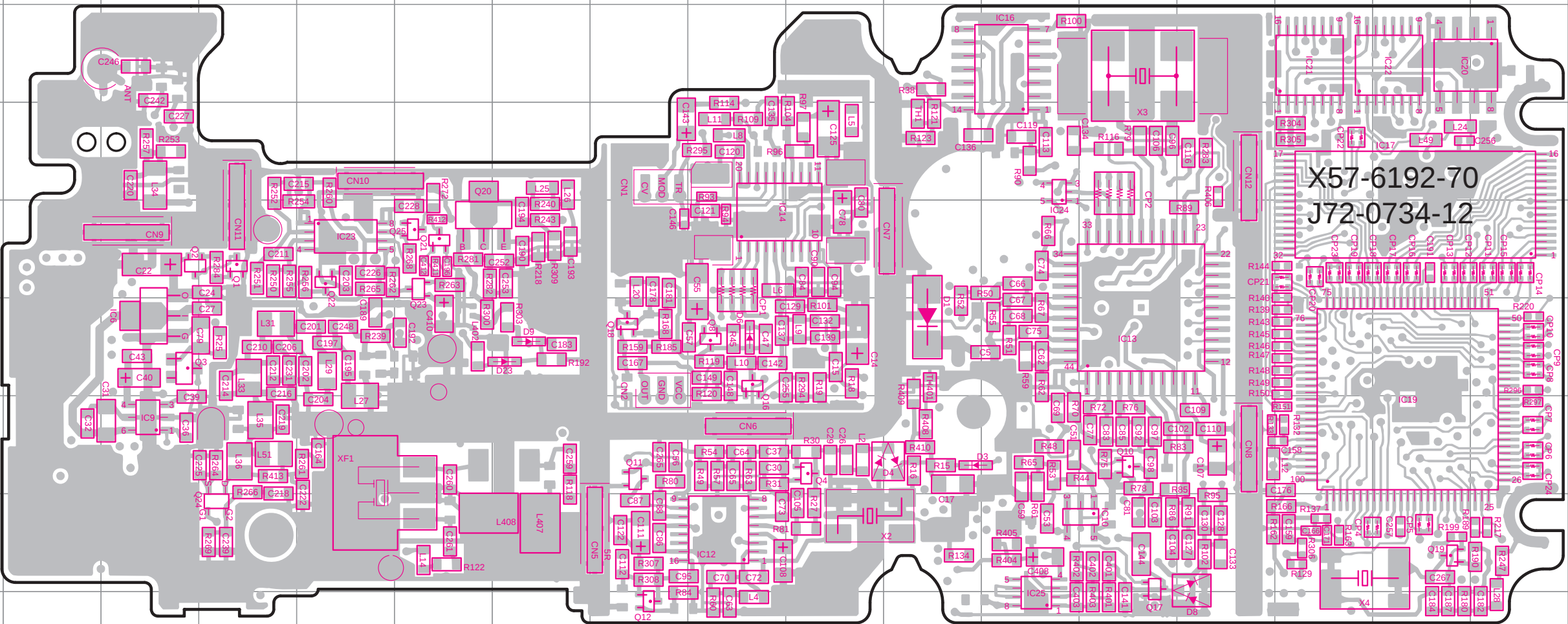
TX-RX UNIT (X57-6192-70) Foil Side View
