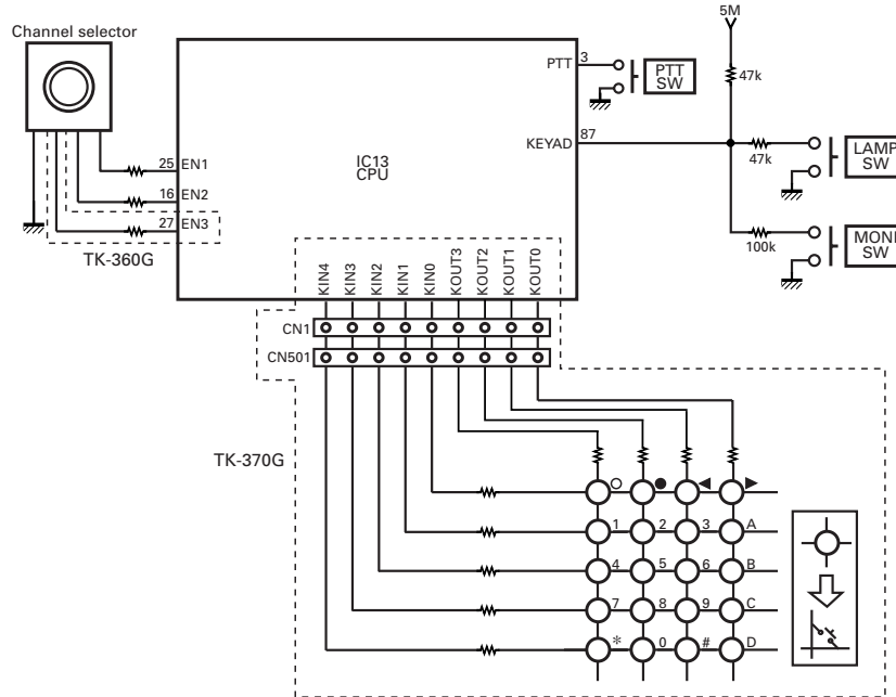
Fig. 10 Control system
