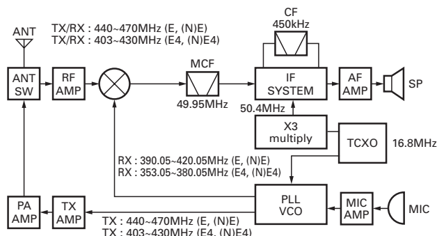
Fig. 1 Frequency configuration
