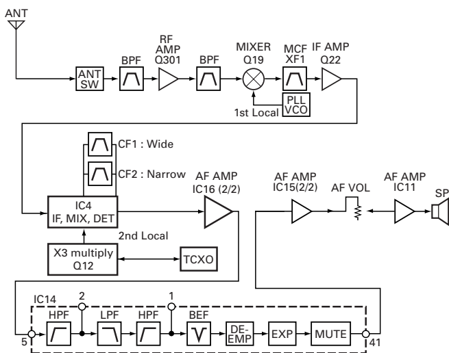
Fig. 2 Receiver section
