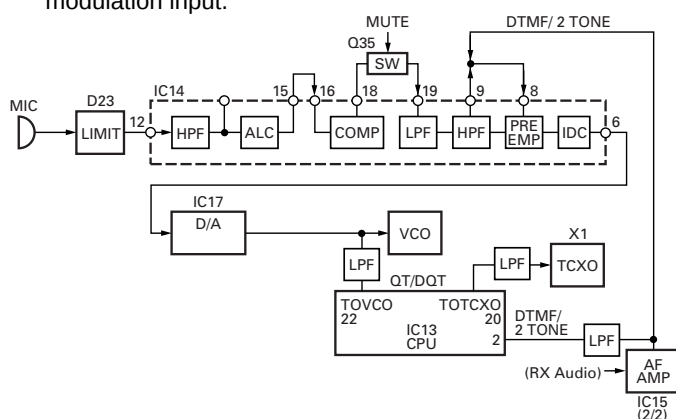
Fig. 7 Microphone amplifier
