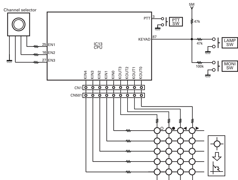
Fig. 10 Control system
