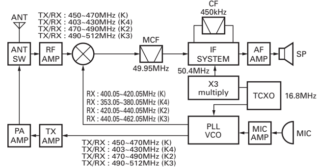
Fig. 1 Frequency configuration
