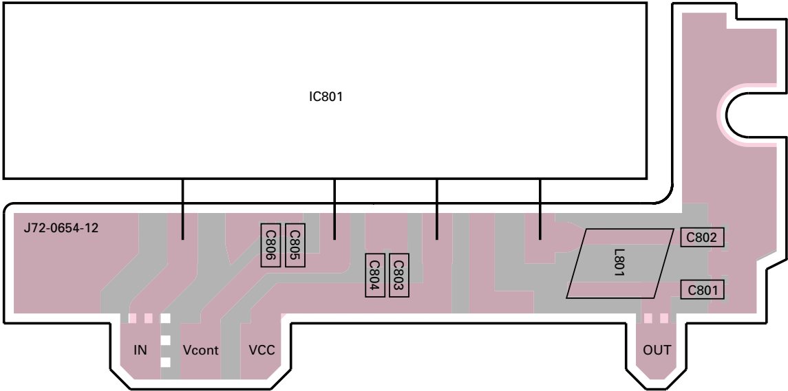
FINAL UNIT (X45-3590-10) Component side view : K3,K6
