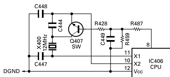
Fig. 13 CPU clock frequency shift
