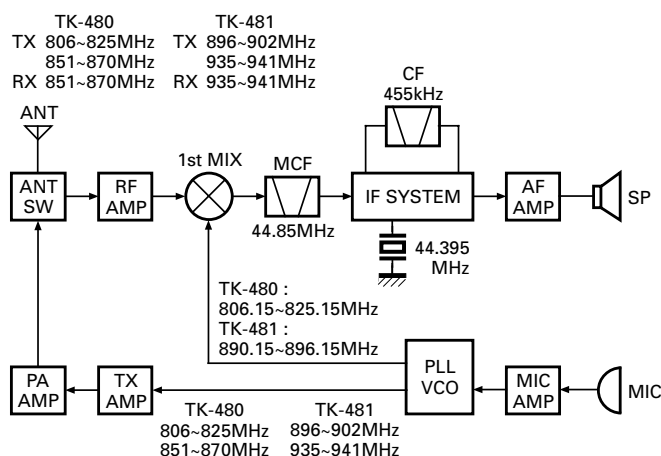
Fig. 1 Frequency configuration
