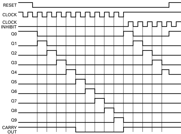
Fig. 11 Decade counter timing chart
