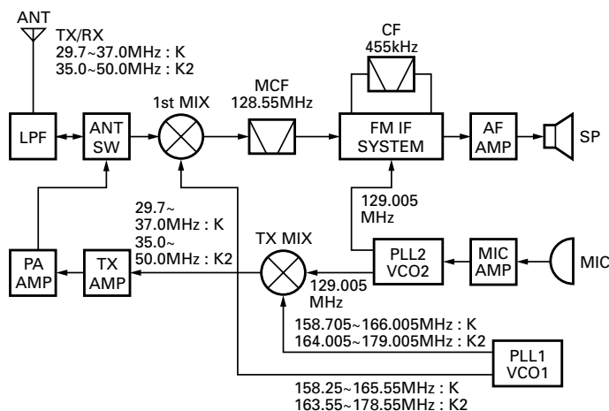
Fig. 1 Frequency configuration
