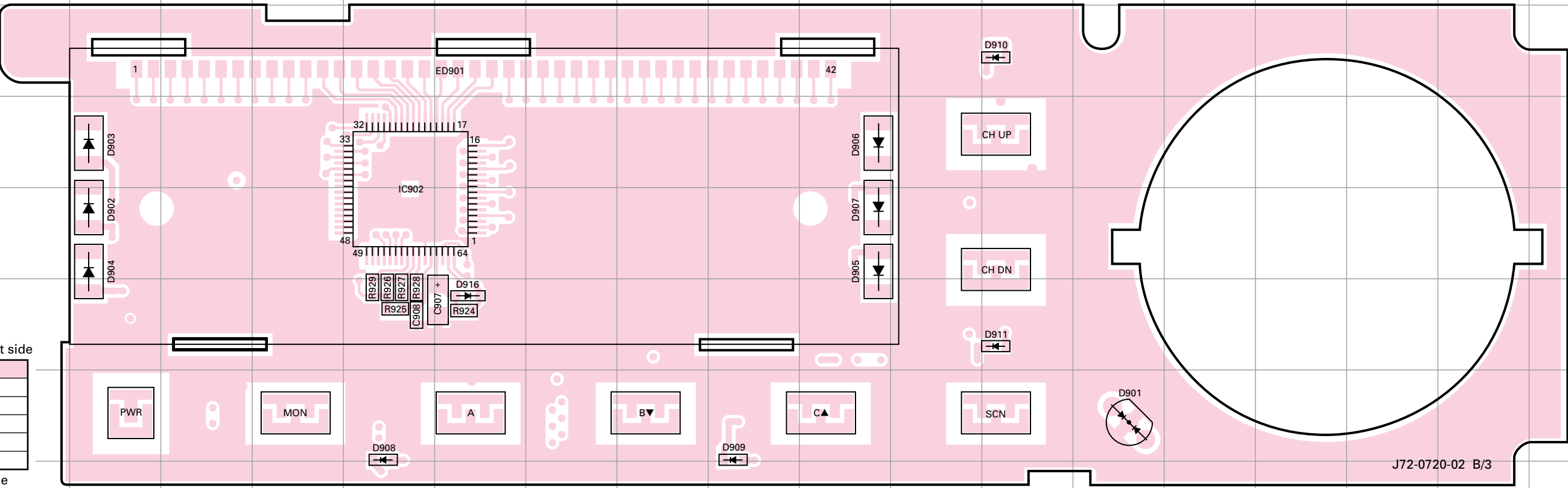
TX-RX UNIT (X57-6100-XX) (B/3) -10 : K -11 : K2 Component side view
