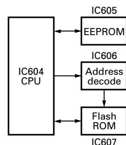
Fig. 9 Memory circuit
