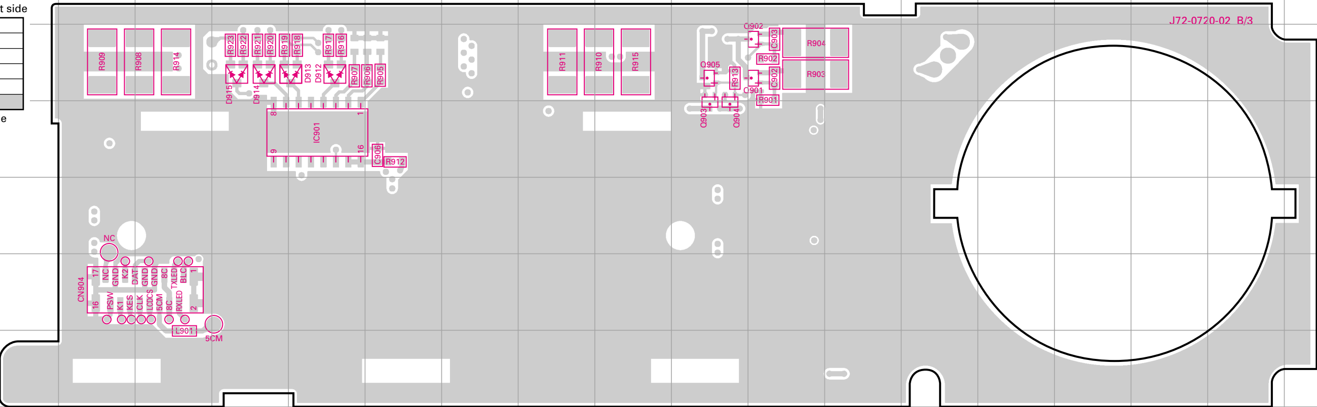
TX-RX UNIT (X57-6100-XX) (B/3) -10 : K -11 : K2 Foil side view
