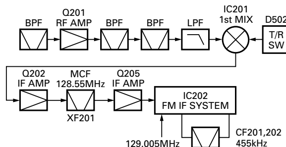
Fig. 2 Receiver section
