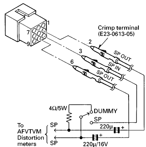
Test cable for speaker output
