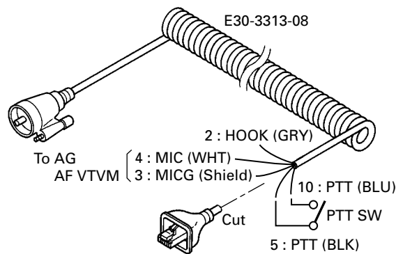
Test cable for microphone input
