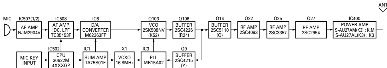
Fig. 8 Transmitter system
