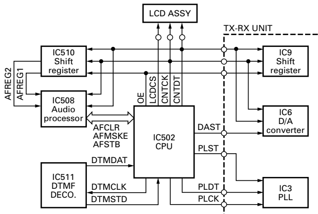
Fig. 10 Control circuit
