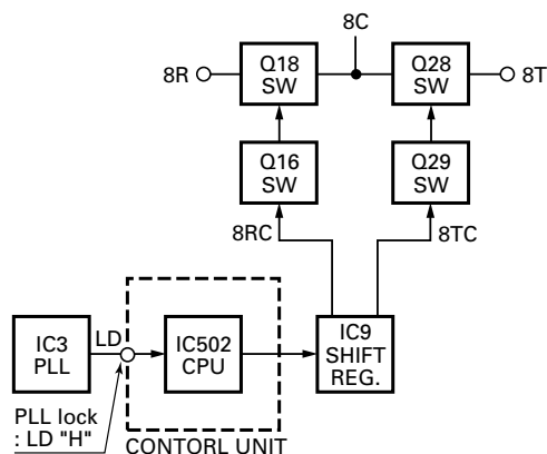
Fig. 7 Unlock circuit
