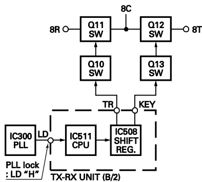
Fig. 7 Unlock circuit
