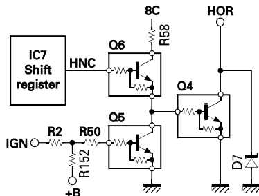
Fig. 15 Horn control
