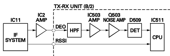
Fig. 5 Squelch circuit
