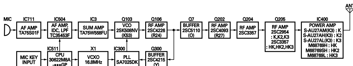
Fig. 6 Transmitter system
