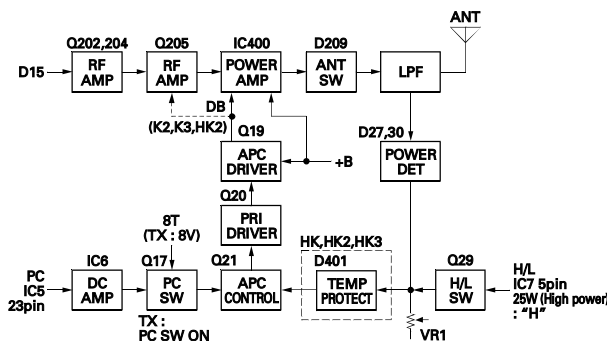
Fig. 8 APC circuit
