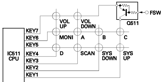
Fig. 12 Key matrix circuit
