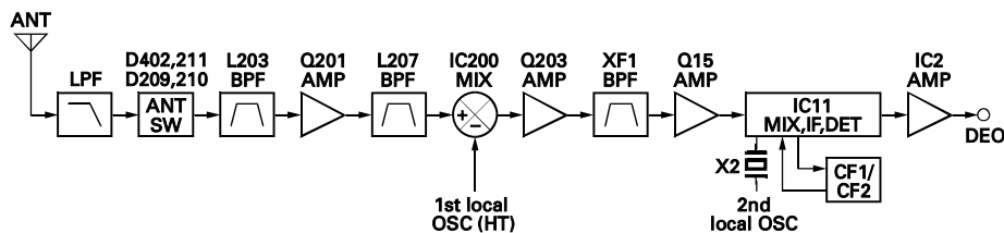
Fig. 2 Receiver system
