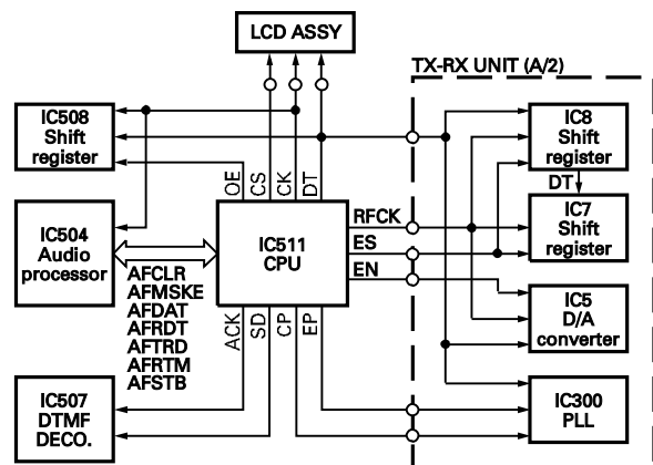
Fig. 9 Control circuit
