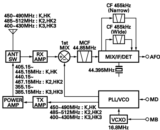
Fig. 1 Frequency configuration
