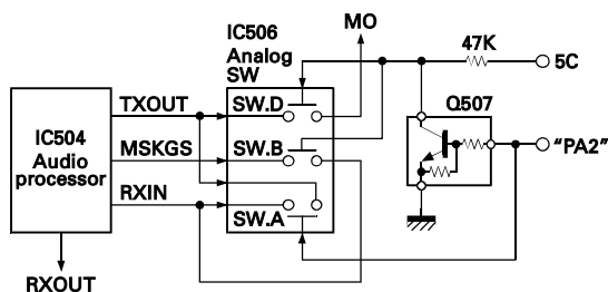
Fig. 16 PA switch
