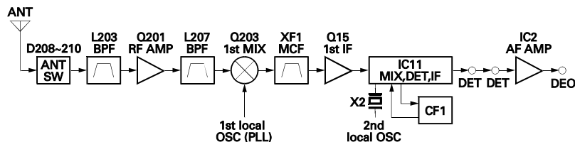
Fig. 2 Receiver system
