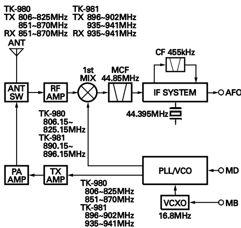
Fig. 1 Frequency configuration
