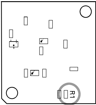
Fig. 11 KAP-1 foil side view
