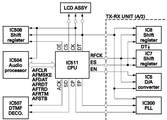
Fig. 8 Control circuit
