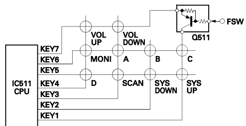
Fig. 11 Key matrix circuit
