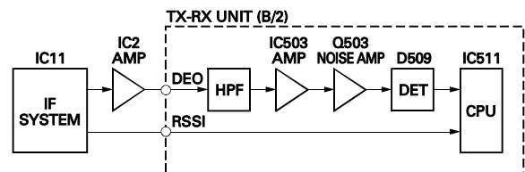
Fig. 4 Squelch circuit
