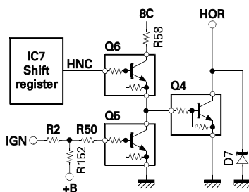
Fig. 14 Horn control
