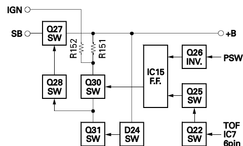
Fig. 16 Power supply circuit
