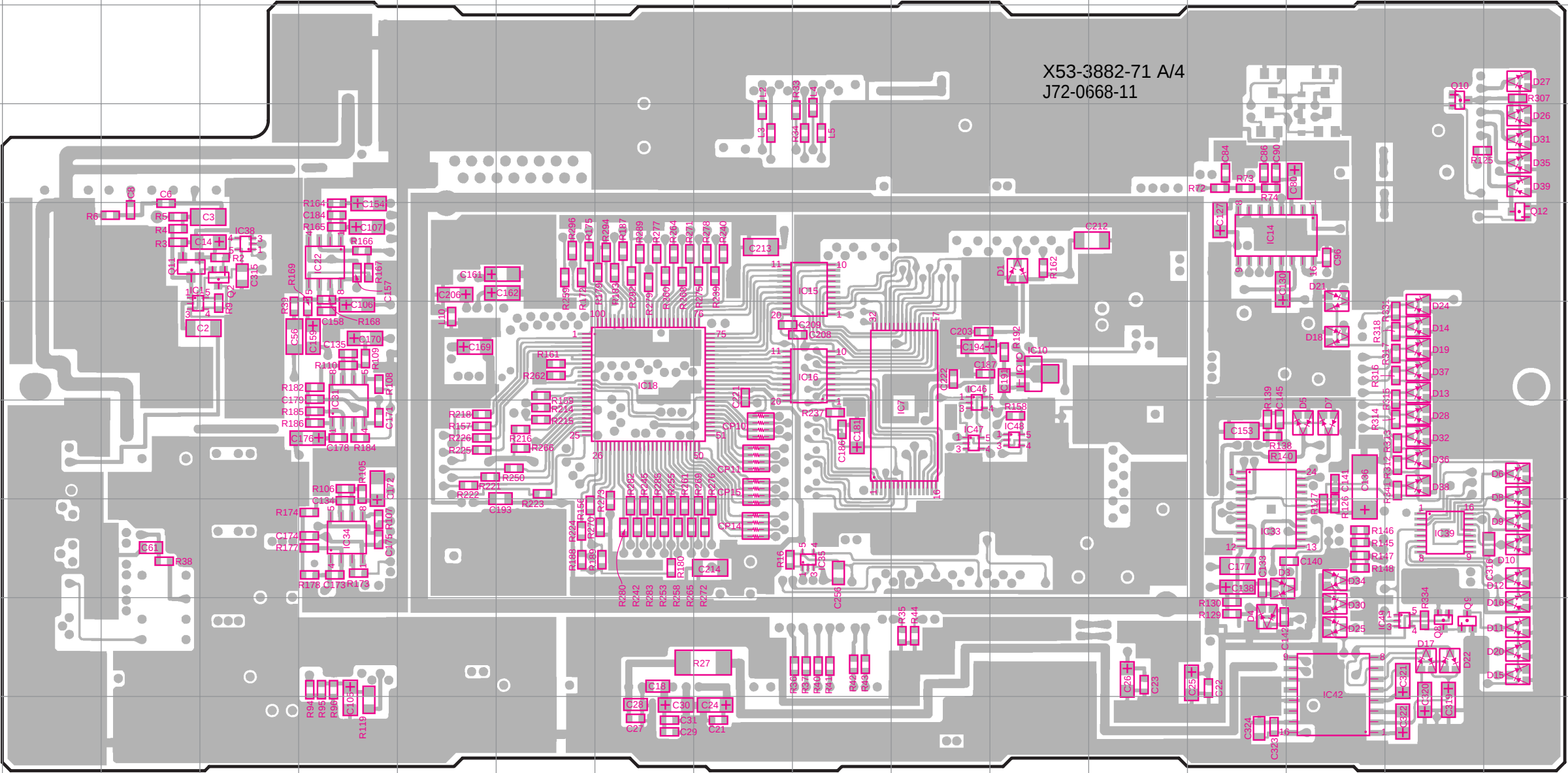
CONTROL UNIT (X53-3882-71) (A/4) Foil Side View (J72-0668-11)
