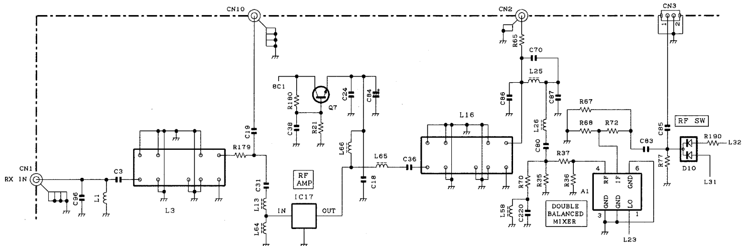
Fig.14 Front-end circuit
