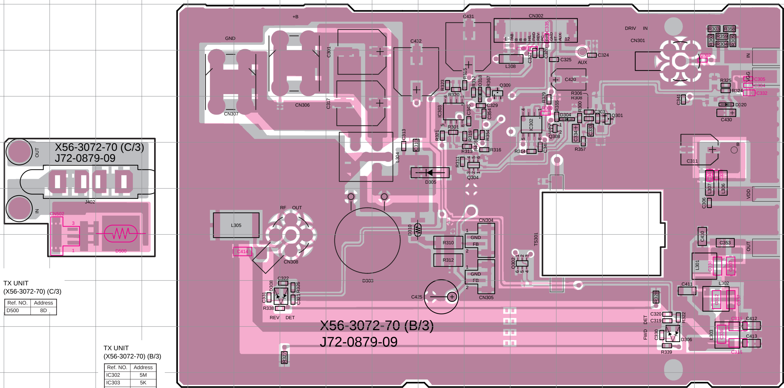
TX UNIT (X56-3072-70) (B/3) (C/3) Component Side + Foil Side View (J72-0879-09)
