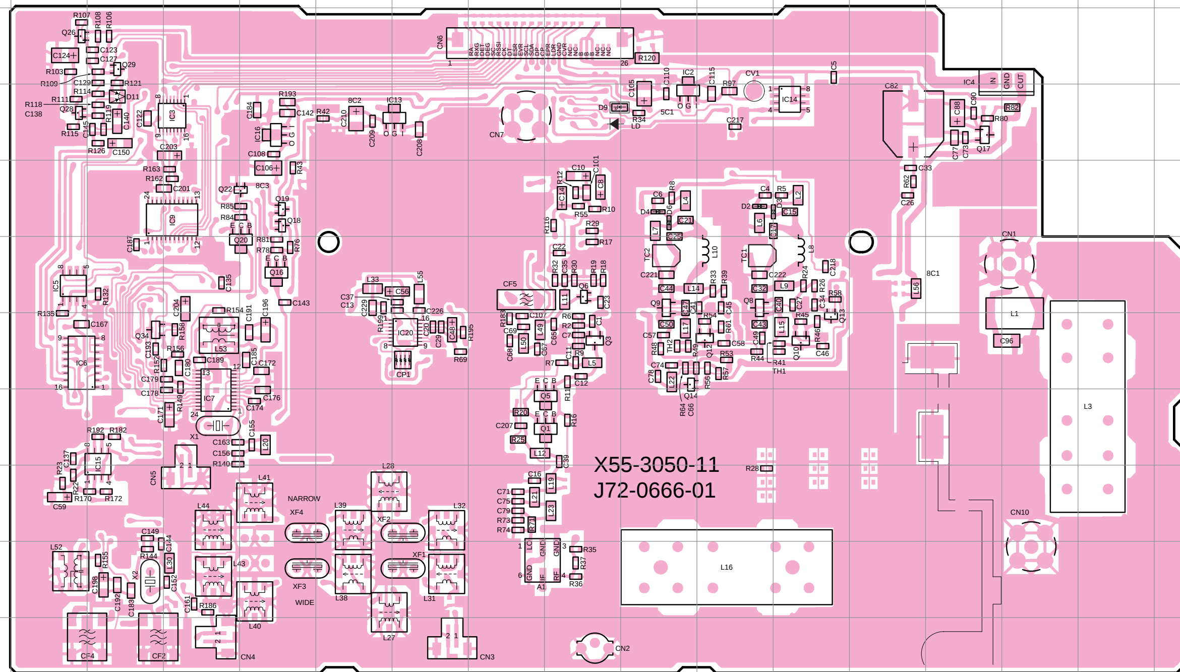
RX UNIT (X55-3050-11) Component Side View (J72-0666-01)
