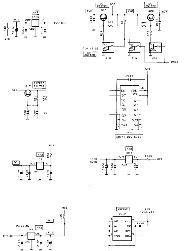
Fig.20 Other circuits
