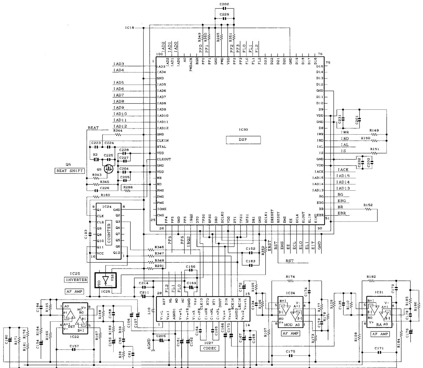
Fig.23 DSP circuit
