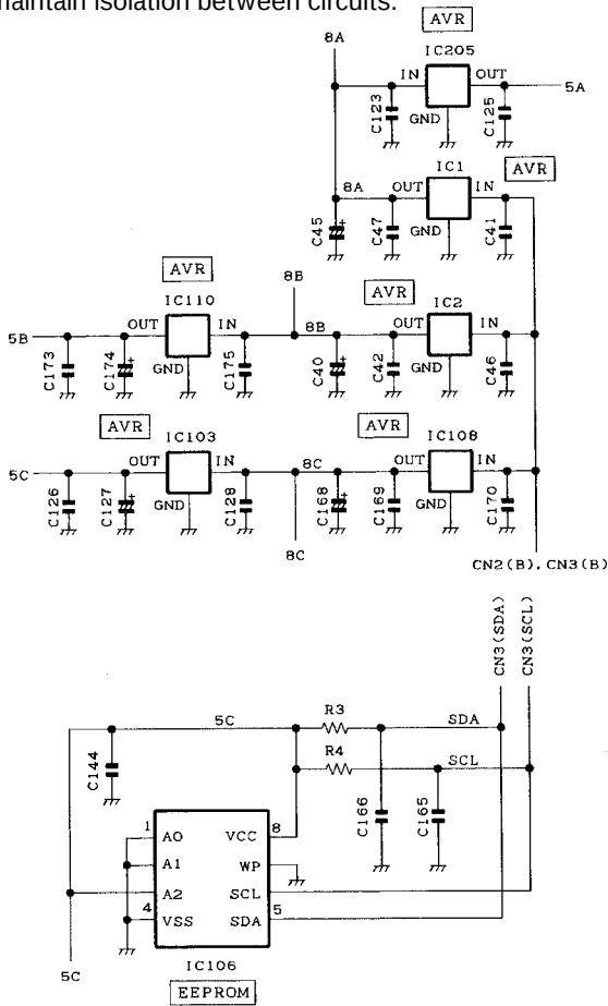
Fig.7 Other circuits
