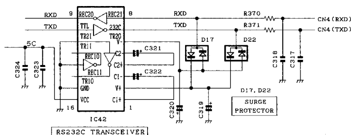
Fig.28 RS-232C circuit
