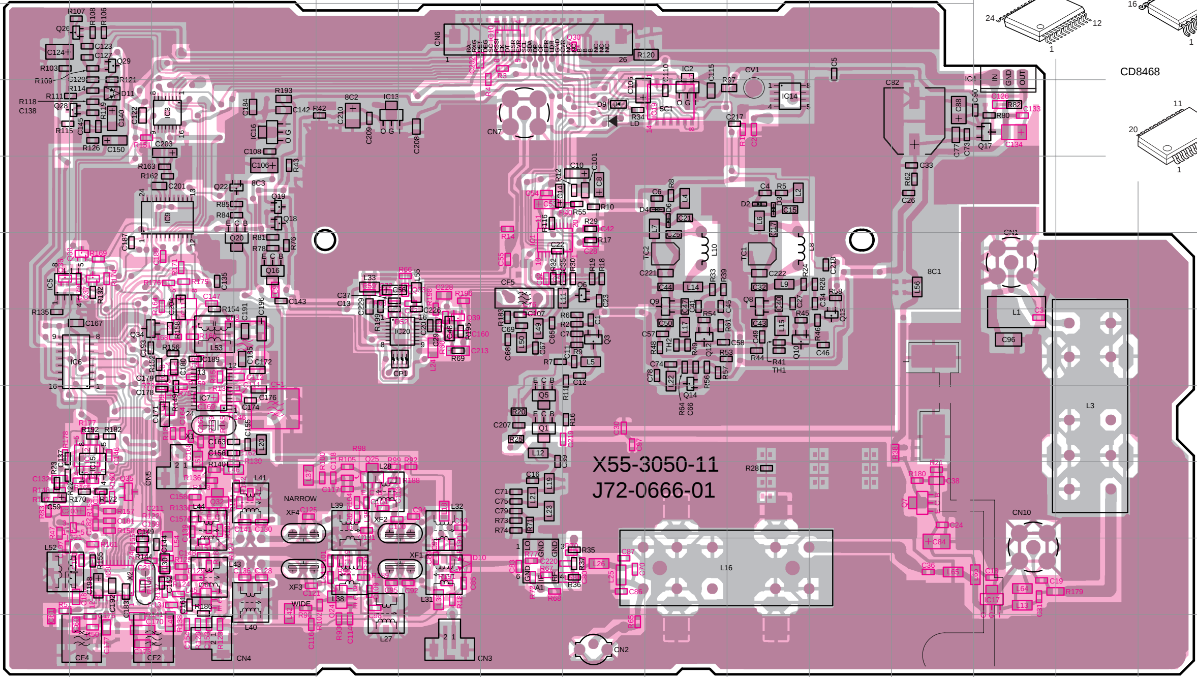
RX UNIT (X55-3050-11) Component Side + Foil Side View (J72-0666-01)
