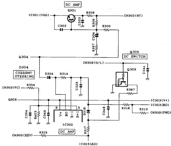
Fig.11 APC circuit
