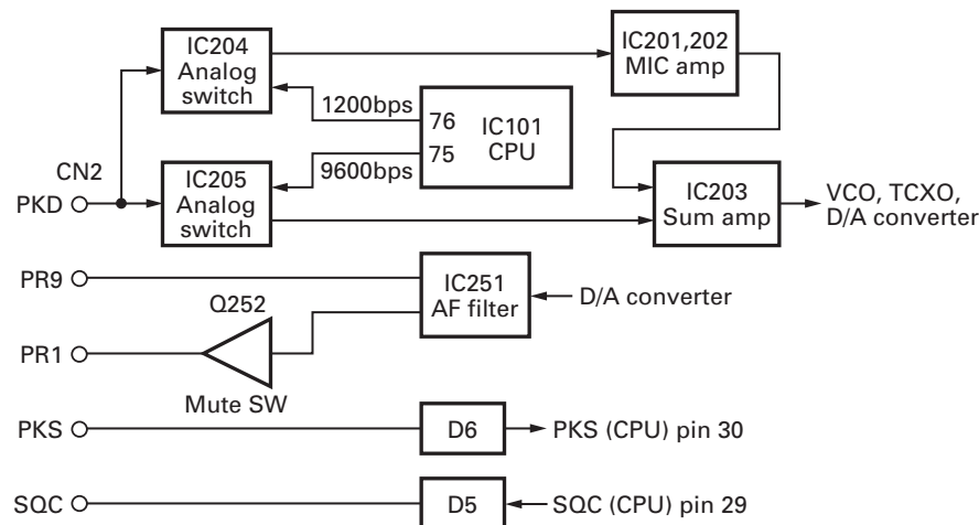
Fog. 17 Data terminal and peripheral circuits
