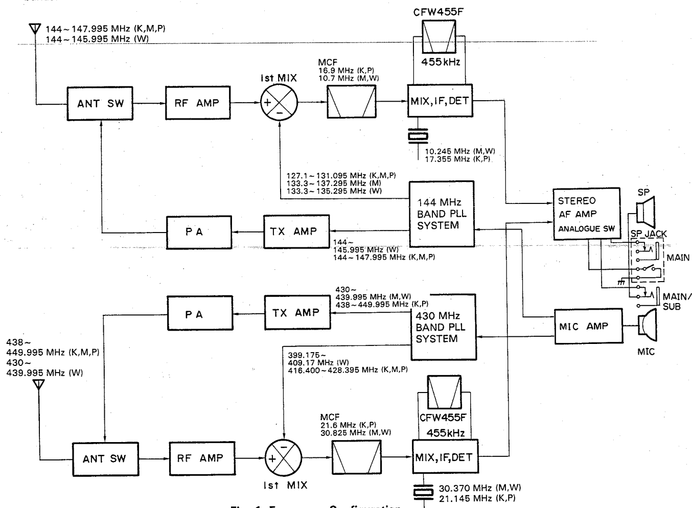
Fig. 1 Frequency Configuration
