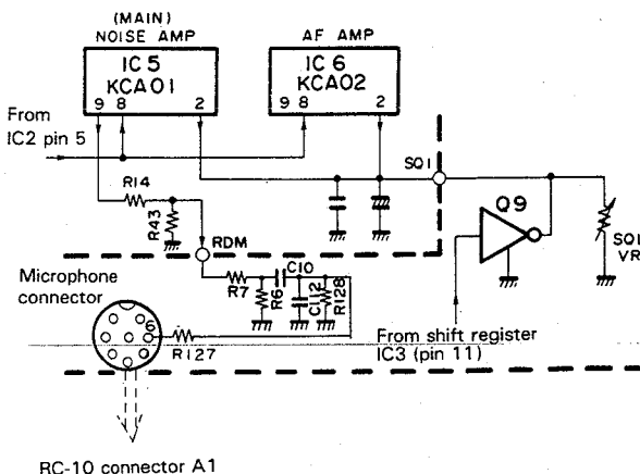
Fig. 22 Squelch Off Circuit
