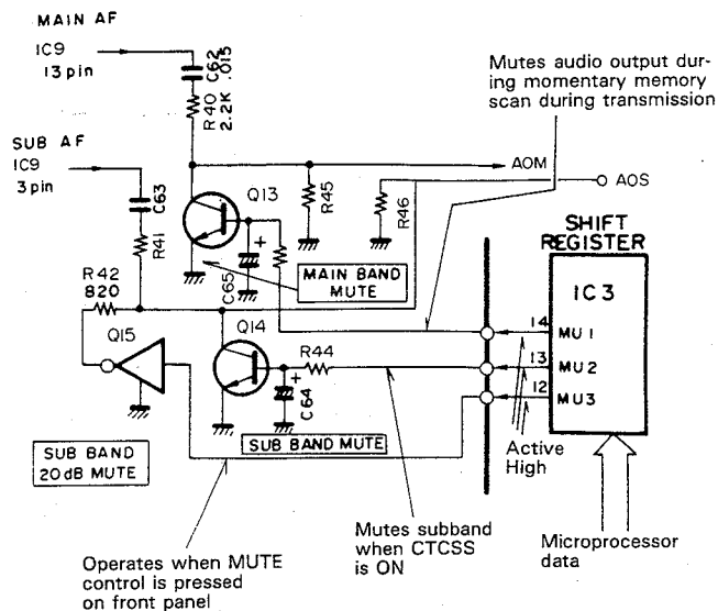
Fig. 8 Mute Circuit
