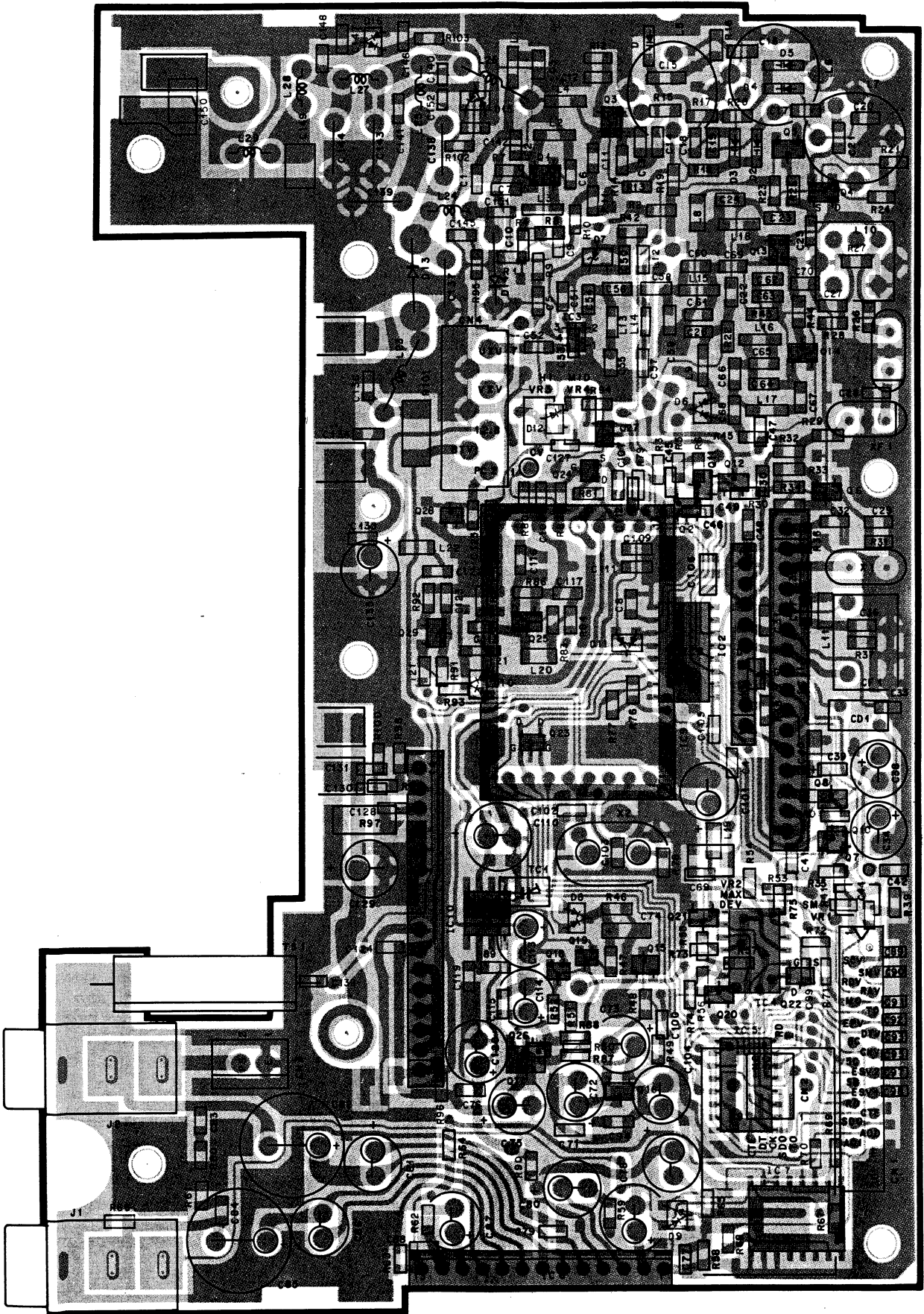
144MHz TX-RX UNIT (X57-400X-XX) (A/4) Component side view 0-11 : K,P 0-21 : M,M2,M3 2-71 : E,E2,E3
