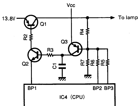
Fig. 15 Dimmer circuit
