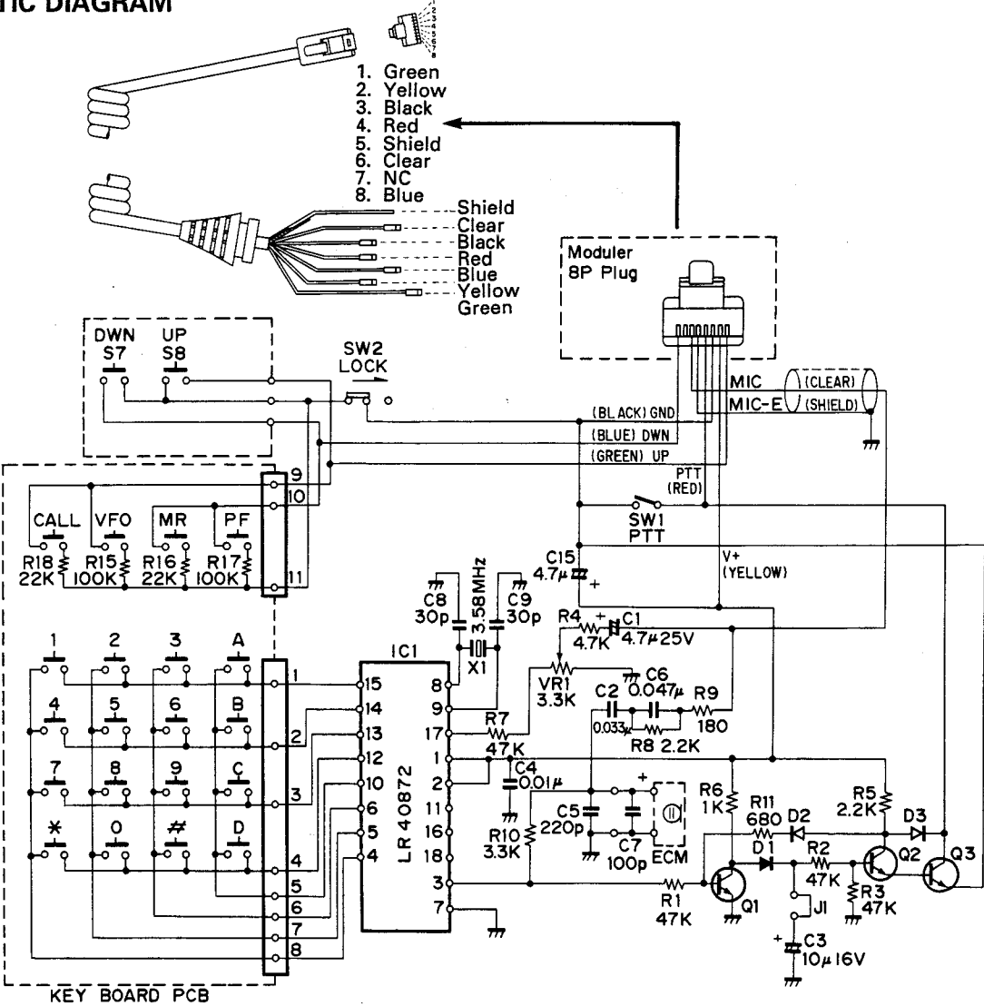
SCHEMATIC DIAGRAM
