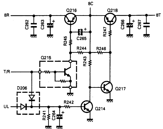
Fig. 6 430MHz band 8T/8R switching circuit and unlock circuit
