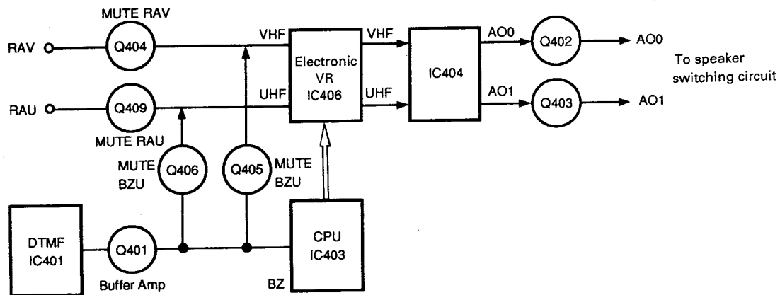
Fig. 7 AF signal system block diagram
