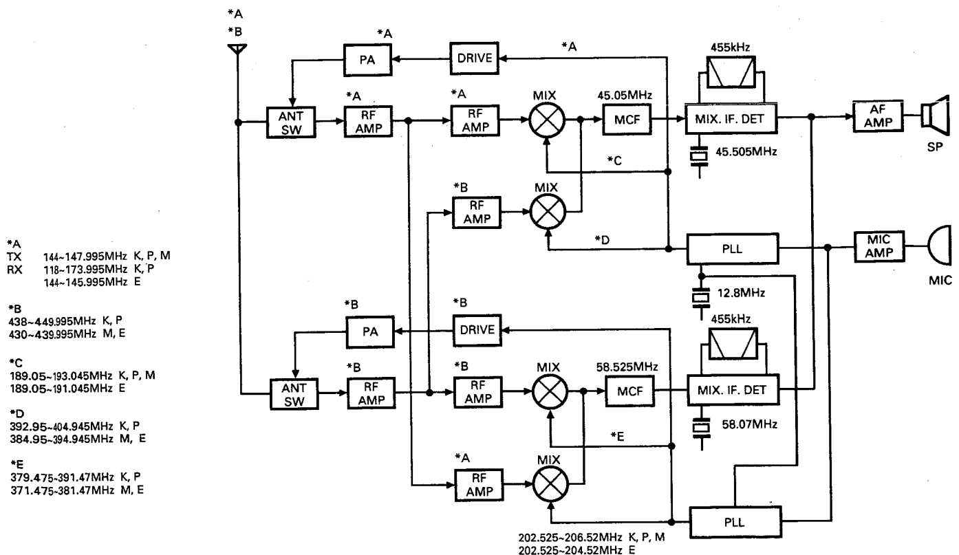
Fig.1 Frequency configuration
