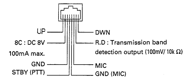
Microphone Socket (on Front Panel)
