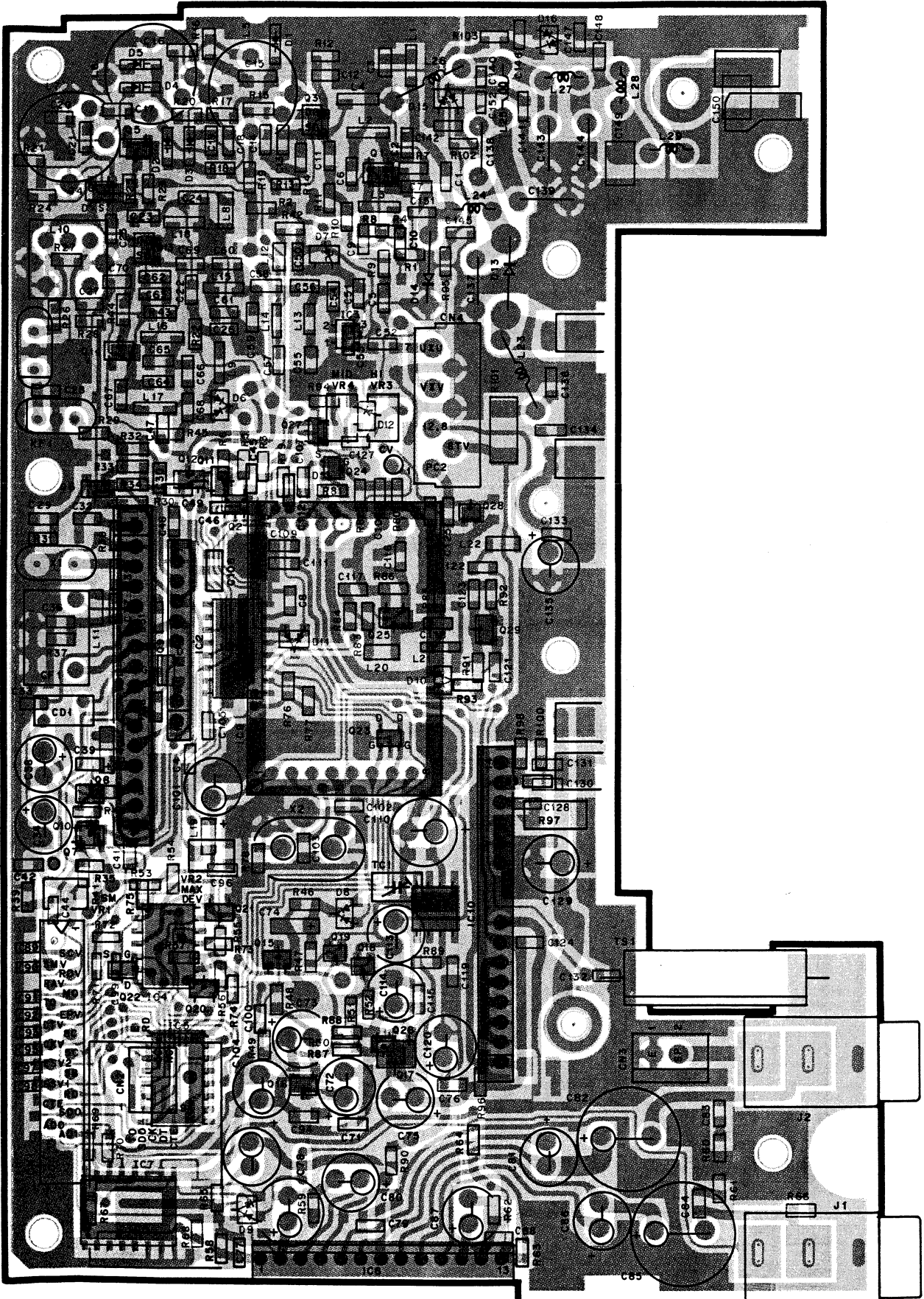
144MHz TX-RX UNIT (X57-400X-XX) (A/4) Foil side view 0-11 : K,P 0-21 : M,M2,M3 2-71 : E,E2,E3
