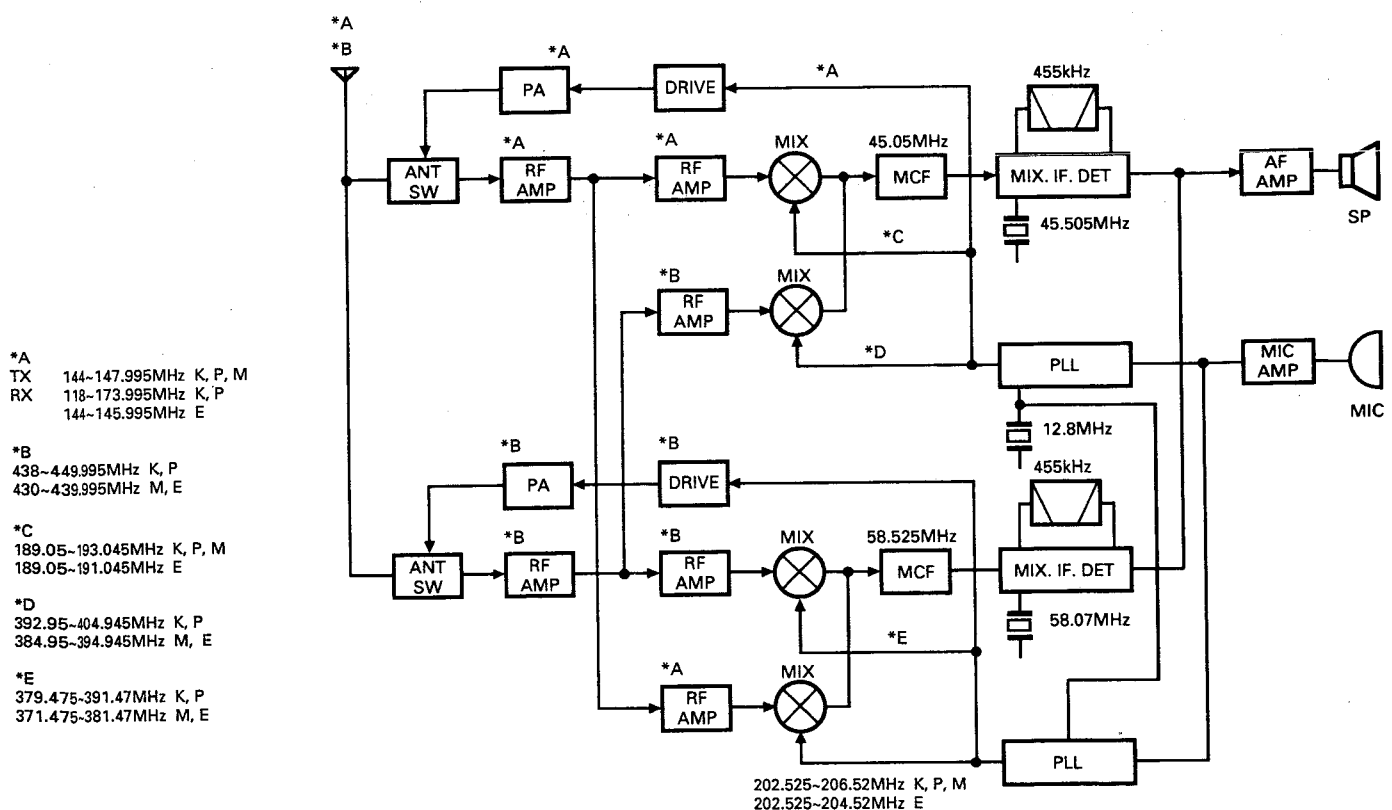
Fig.1 Frequency configuration
