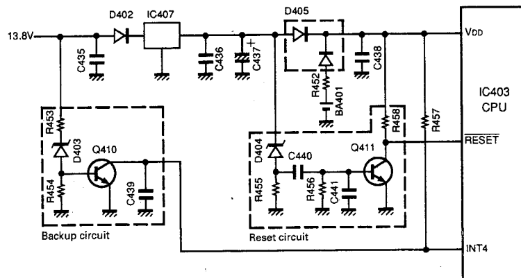
Fig. 12 Reset and backup circuits
