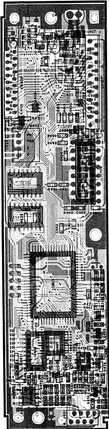
CONTROL UNIT (X57-400X-XX) (C/4) Component side view
