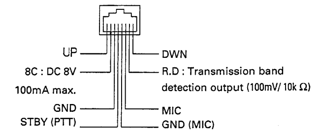
Microphone Socket (on Front Panel)
