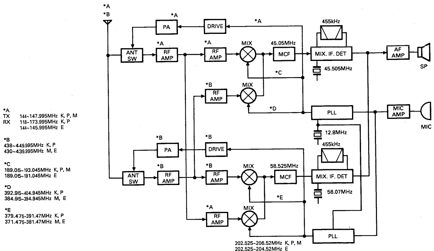
Fig.1 Frequency configuration
