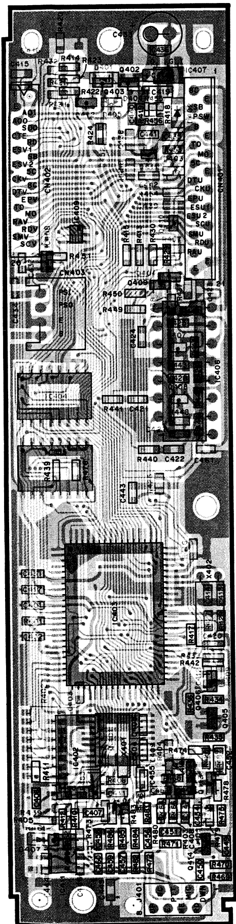
CONTROL UNIT (X57-400X-XX) (C/4) Component side view 0-11 : K,P 0-21 : M,M2,M3 2-71 : E,E2,E3
