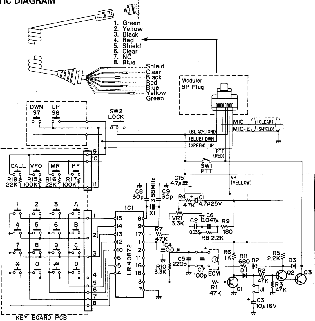
SCHEMATIC DIAGRAM
