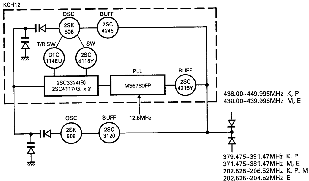
Fig. 17 430MHz band PLL block diagram
