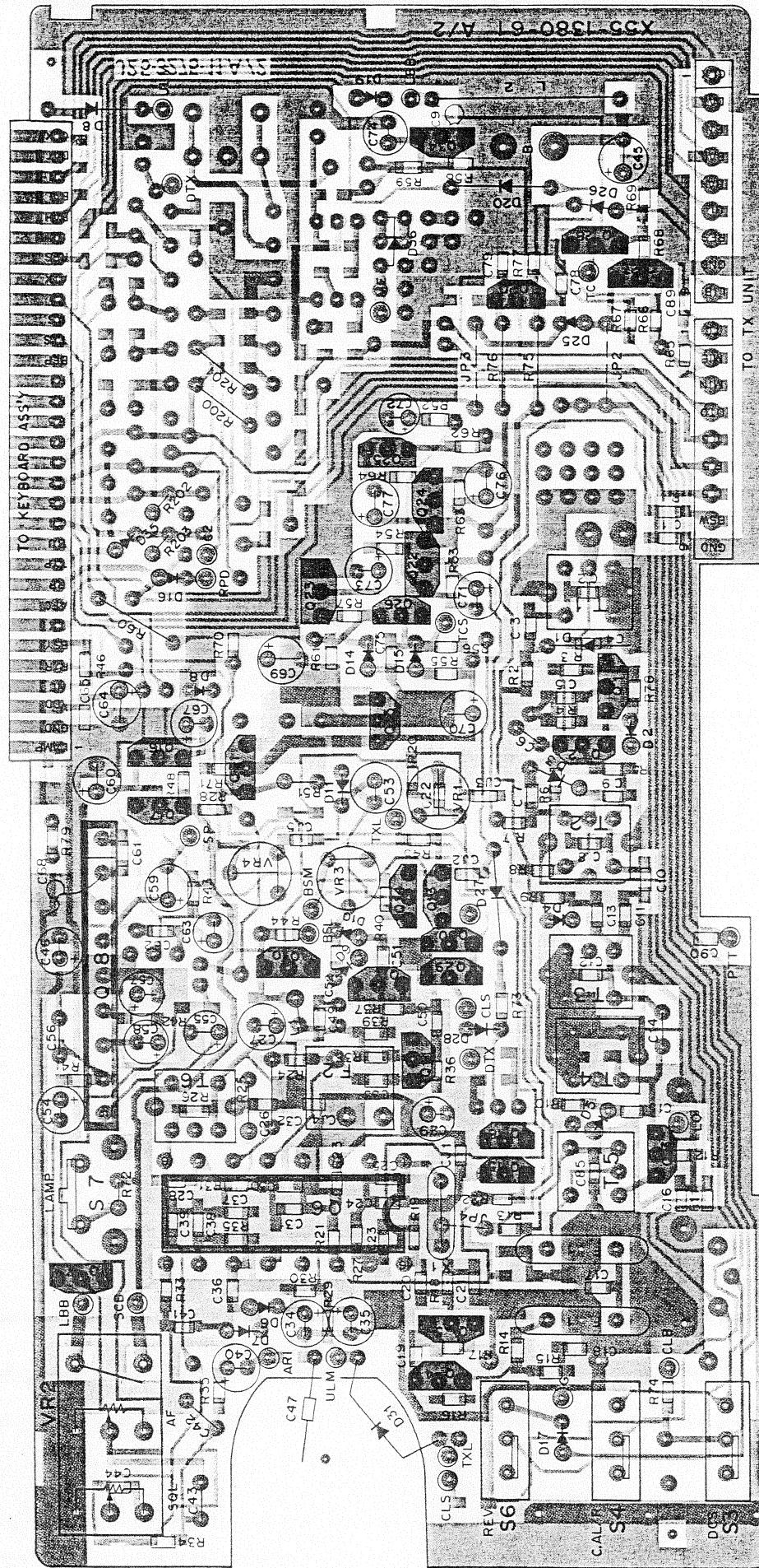
RX UNIT (X55-1380-61) (A/2) (T,W) Component side view
