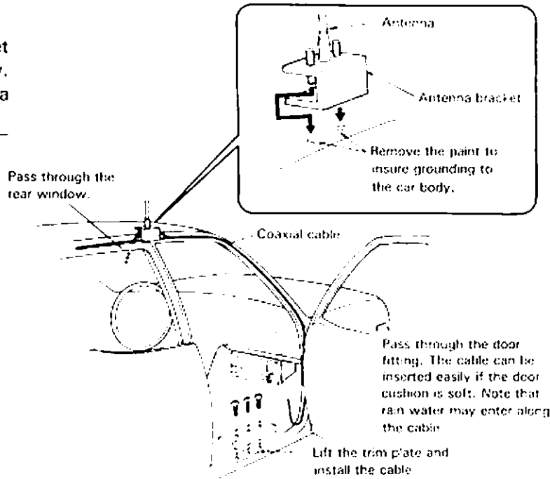
Coax. cable routing
