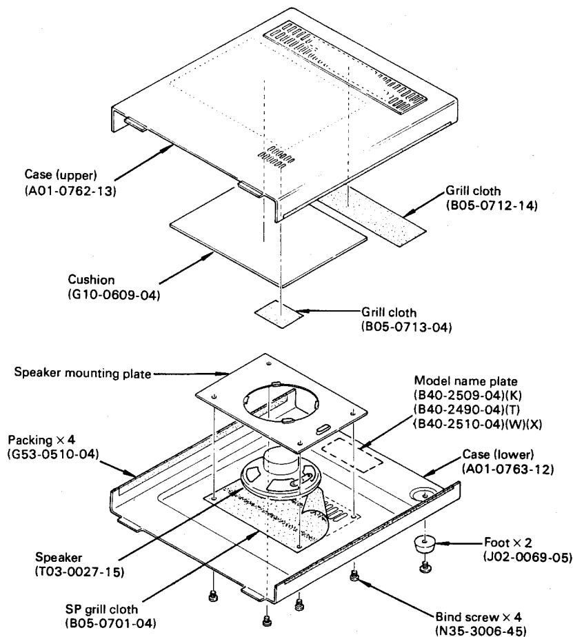
Fig. 12 Case disassembly
