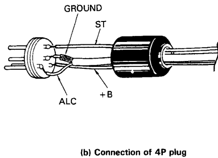
Fig. 3-8 Aux terminal connection
