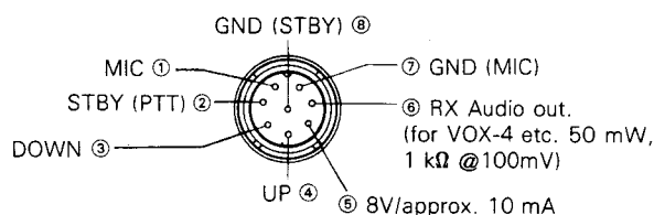
MIC connector (Front view)
