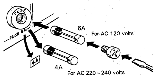
Fig. 3-1B Fuse replacement
