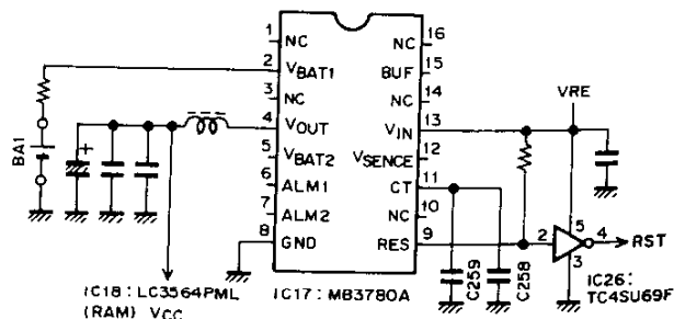
Fig. 26 System reset and RAM backup
