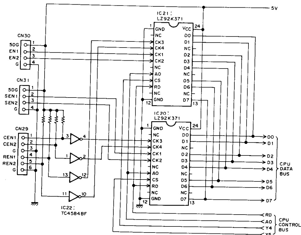
Fig. 25 Encoder circuit
