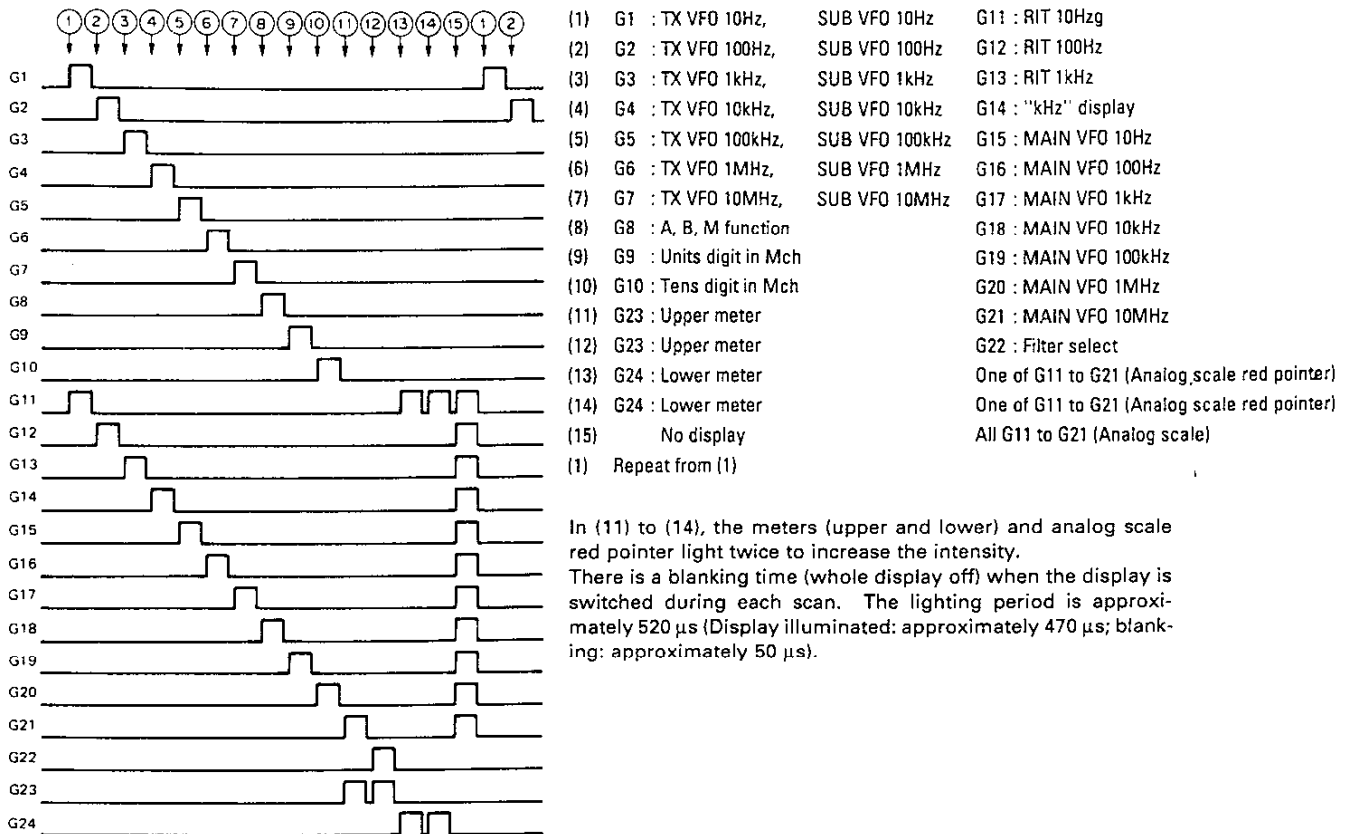
Fig. 29 Timing chart for display lighting (grid only)
