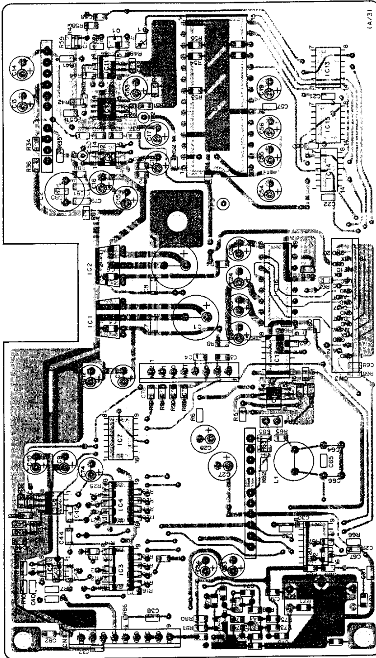
DSP UNIT (X53-3390-00) Foil side view
