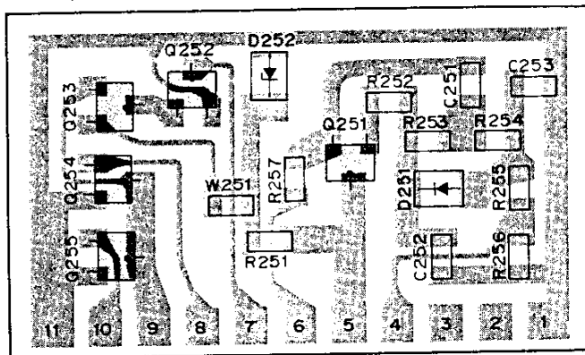
ALC (X59-3700-00) Component side view
