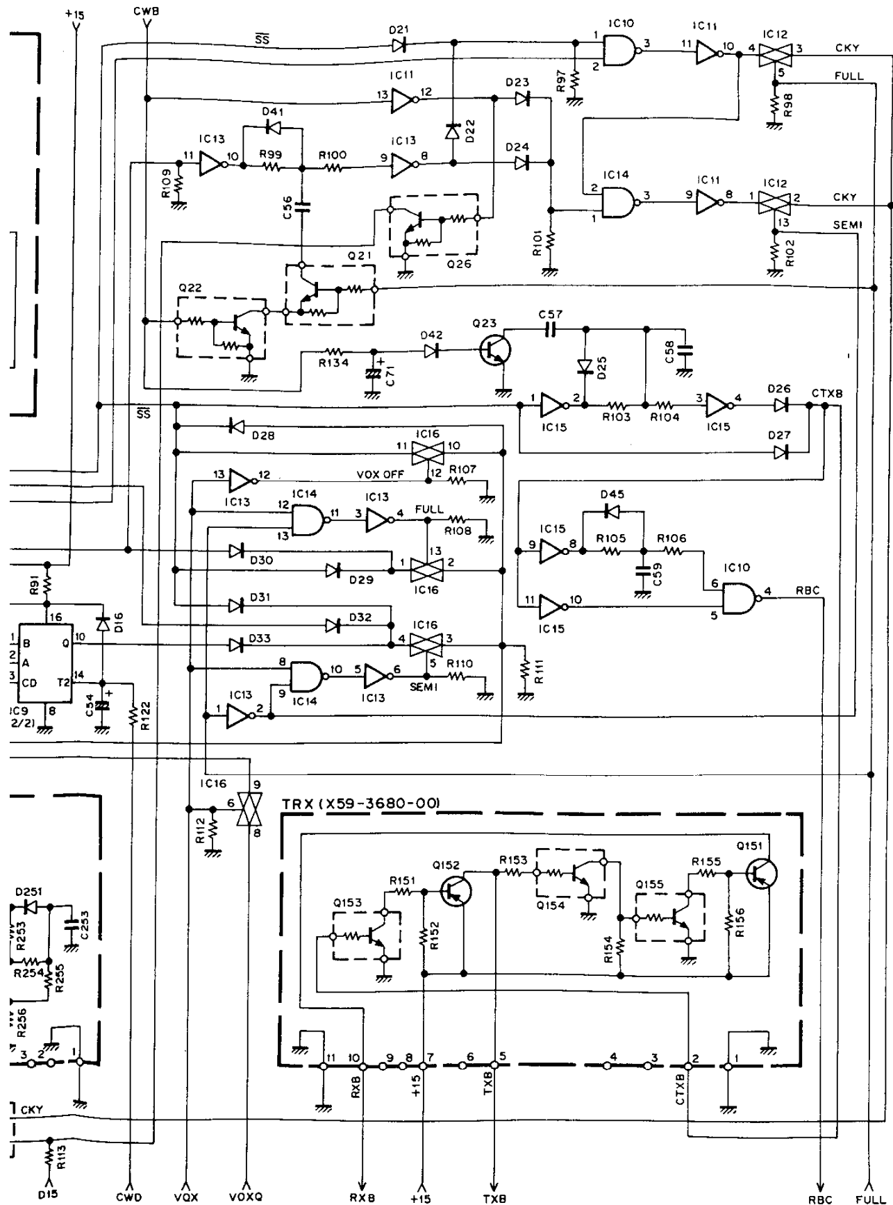
0 Standby circuit
