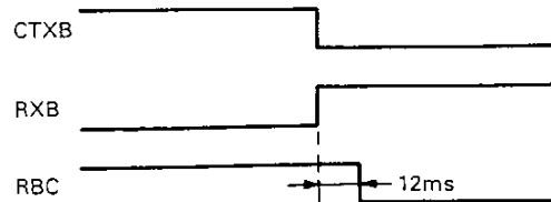
Fig. 18 RBC generation
