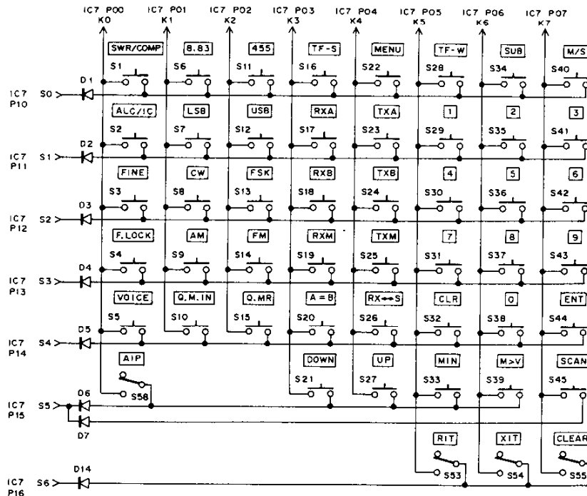
Fig. 31 Key matrix
