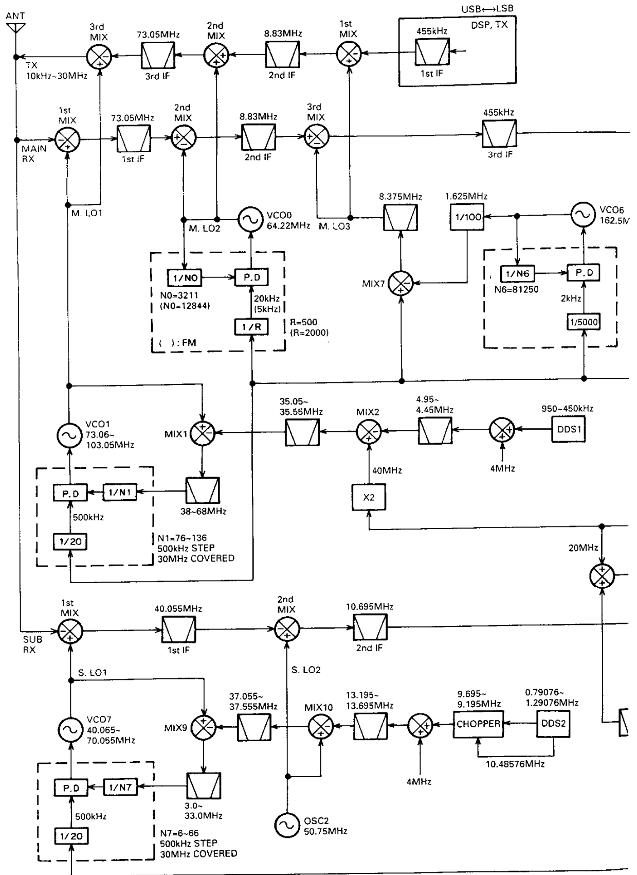
Fig. 2 PLL syst
