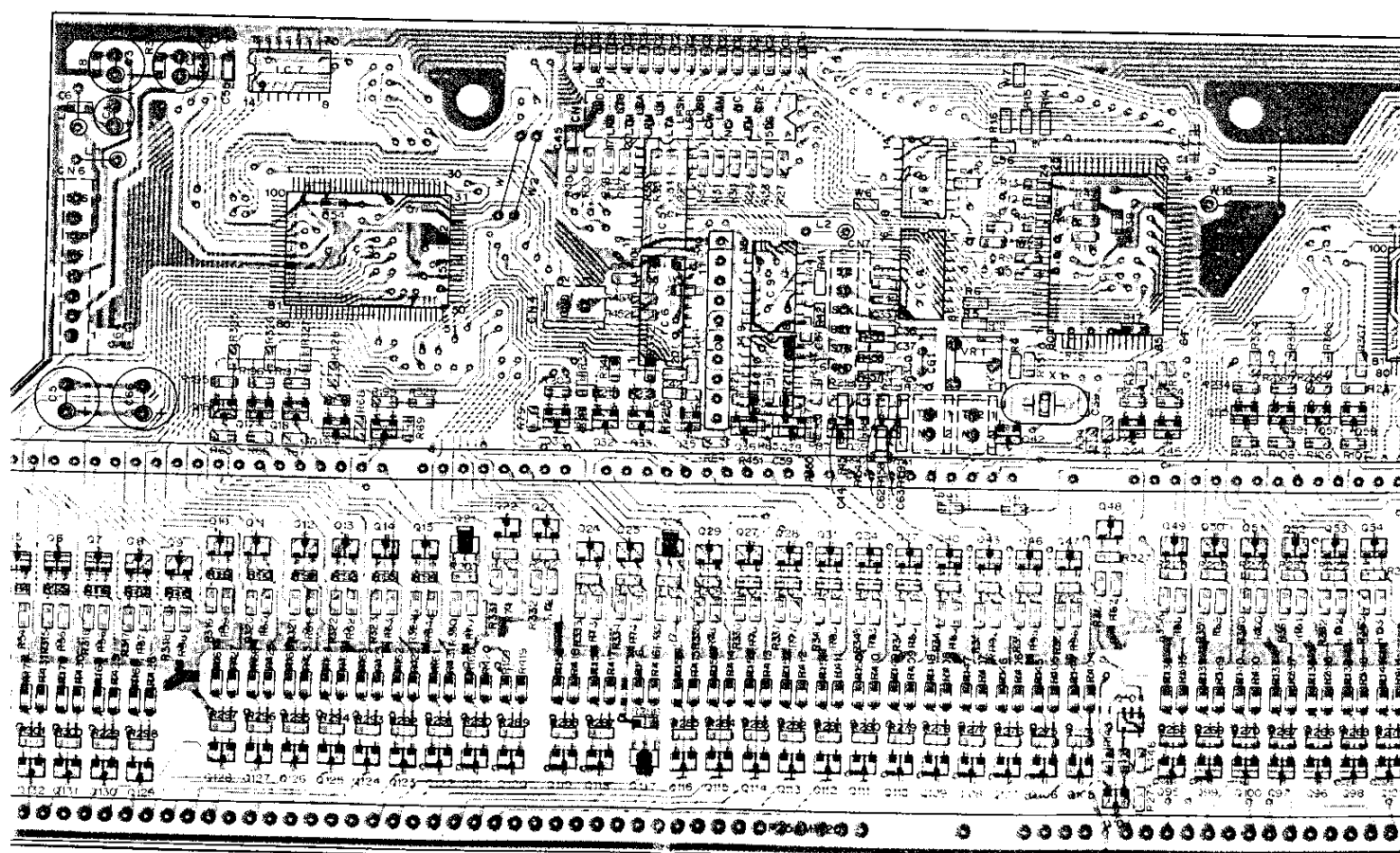
54-3080-01) Foil side view
