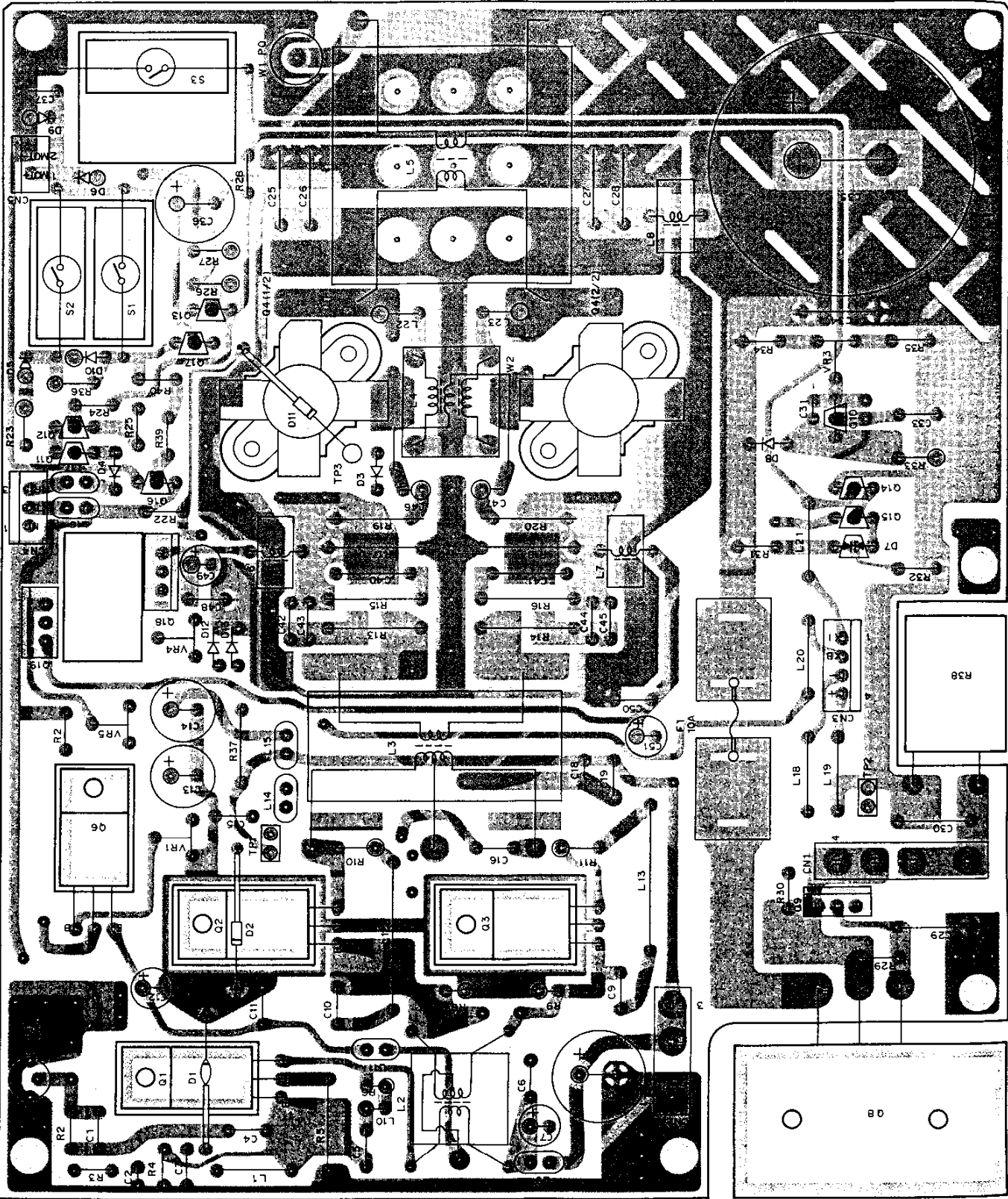
FINAL UNIT (X45-3450-00) Component side view
