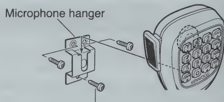
Microphone hanger screw (3 mm x 10 mm)
