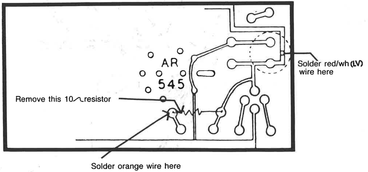
FIGURE NO. 3b Metering Board
