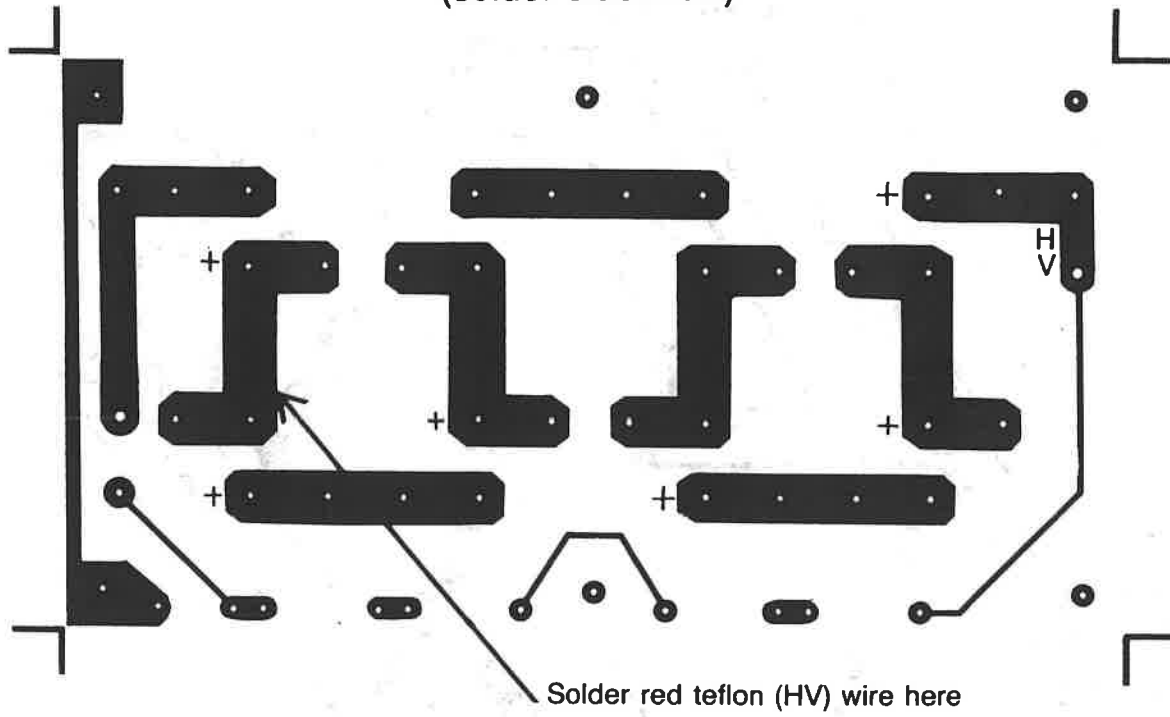
FIGURE NO. 3a (solder-side view)
