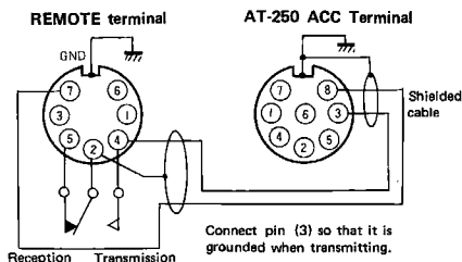
Fig. 3 View from the rear panel
