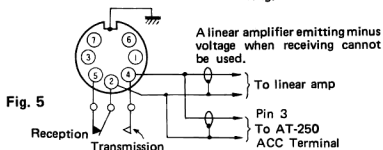
Rear view of the connector
