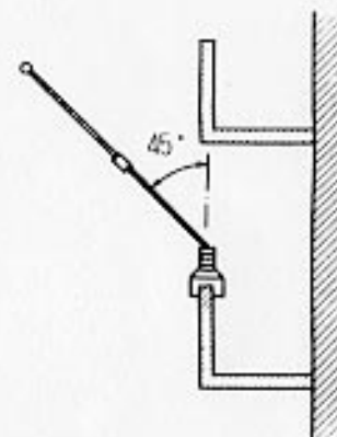
Fig. 3 Installation on the Outside of Concrete Wall
