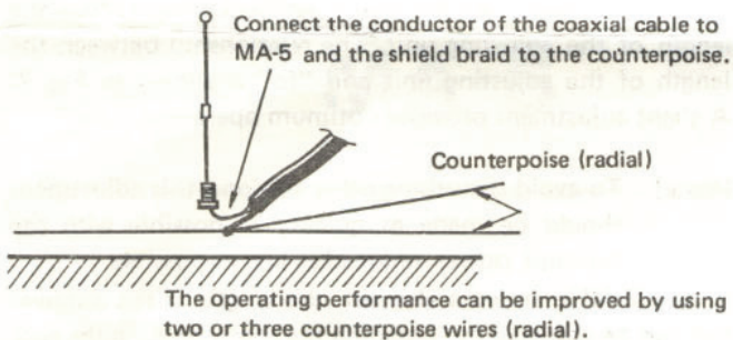
Fig. 4 Field Operation
