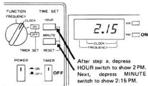
Fig. 3-6 Setting at 2:15 PM
