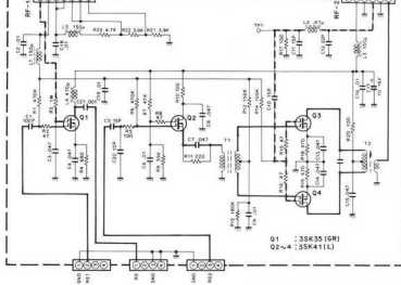
PLL ASSY UNIT (X60-1010-01)
