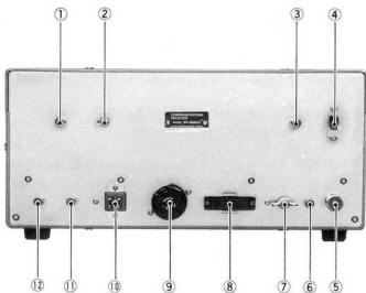
Fig. 3.2 Rear Panel
