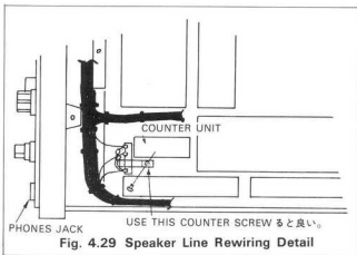
Fig. 4.29 Speaker Line Rewiring Detail
