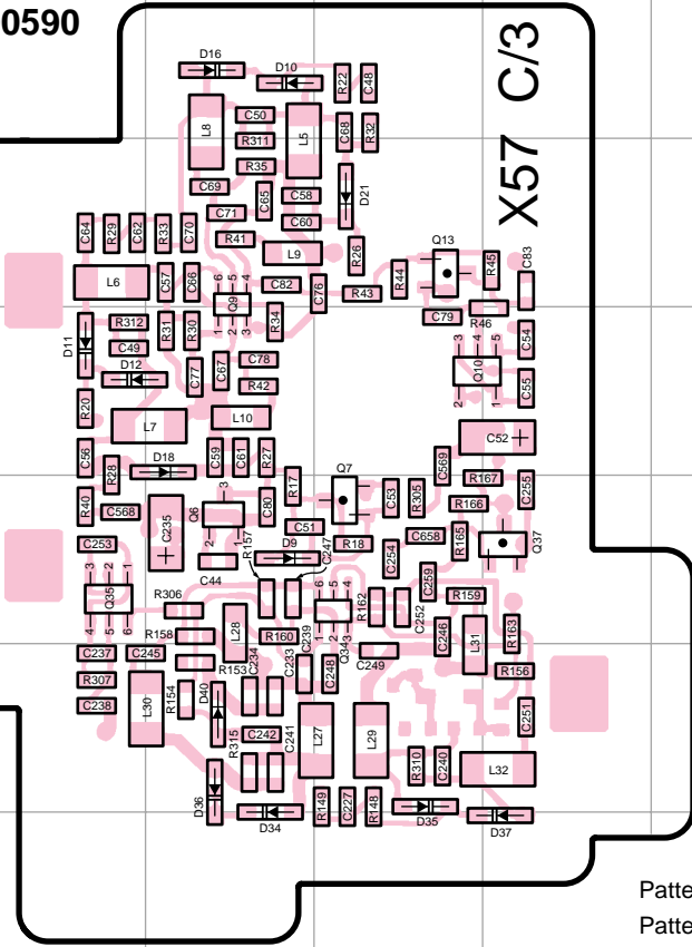
VCO SECTION(C/3) (Component side)
