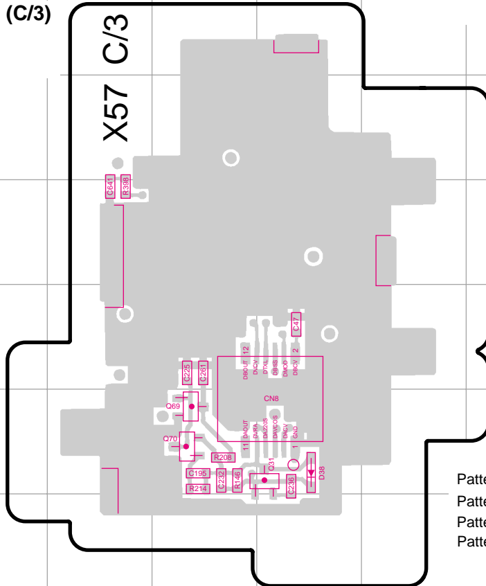
VCO SECTION(C/3) (Foil side)
