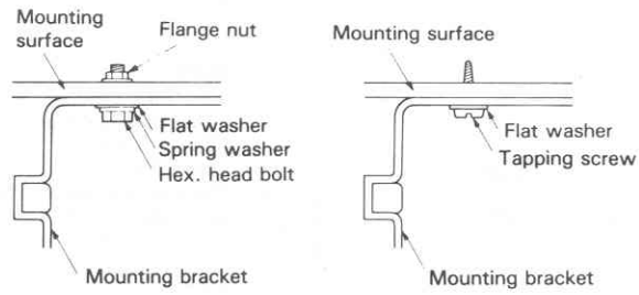
Fig. c Mounting bracket installation
