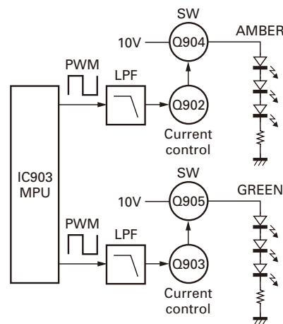
Fig. 14 Brightness circuit
