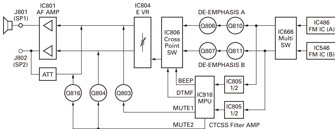
Fig. 4 Audio circuit
