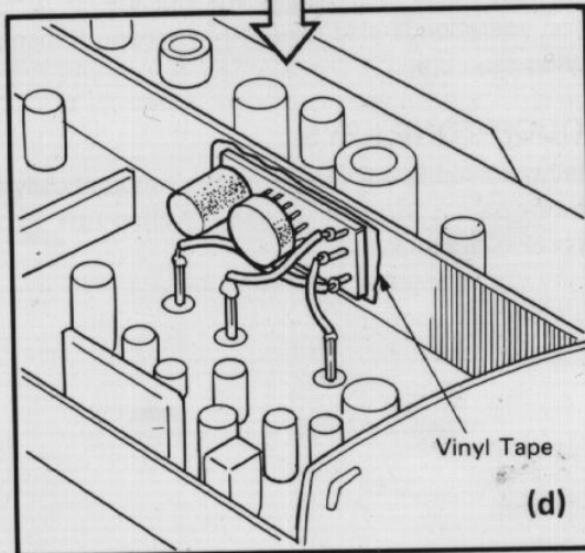
Fig. 4-1 Installing a TONE unit.
