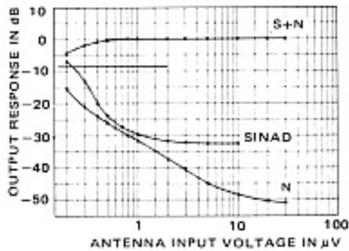
SIGNAL TO NOISE RATIO, OUTPUT LEVEL VS ANTENNA INPUT VOLTAGE
