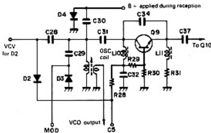
Fig.4 VCO circuit
