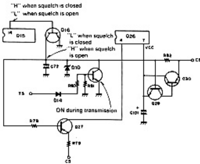
Fig.3 Squelch circuit
