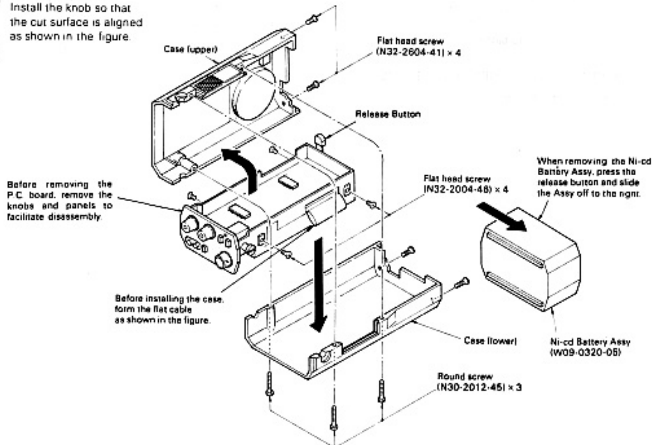
Fig. 14 Case Removal
