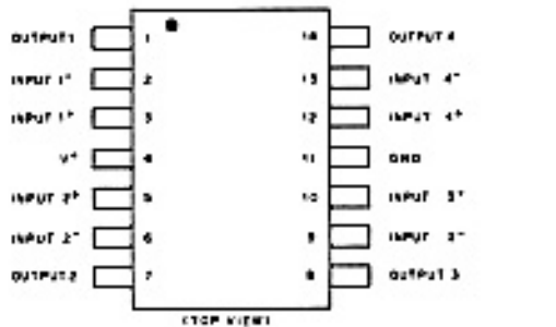
Fig.7 NJM2902N (PLL UNIT Q25) K TYPE ONLY
