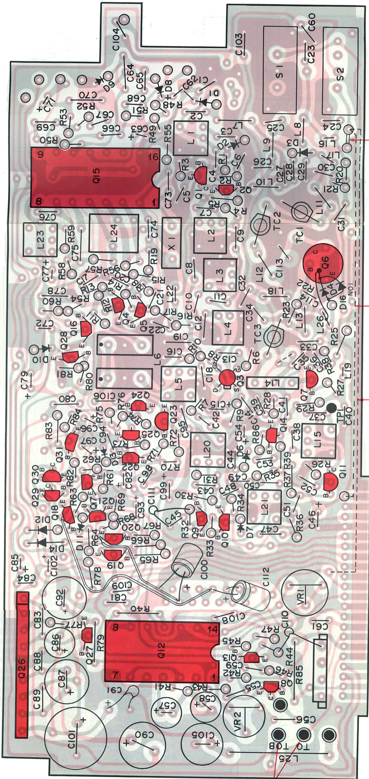
▲ TX-RX UNIT (X44-1460-10,-61,-51) Foil Side View
