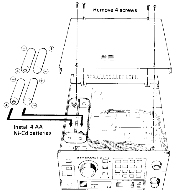
Fig. 1-4 Battery Back-up
