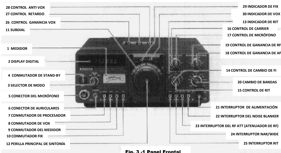
Fig. 3 -1 Panel Frontal
