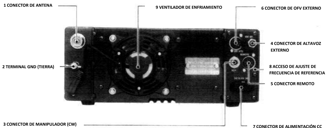
Fig. 3-2 Panel trasero
