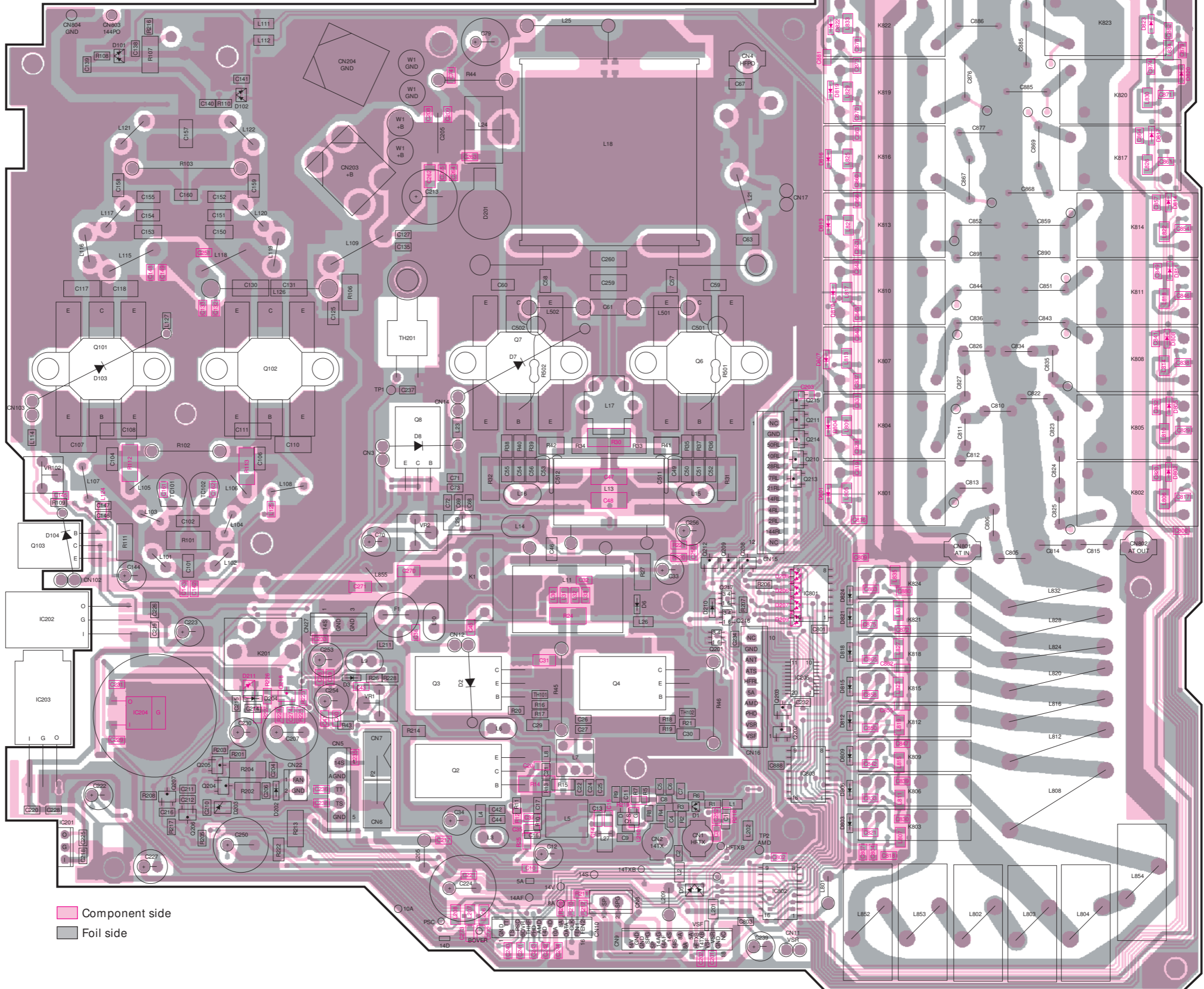
FINAL UNIT (X45-360X-XX) (A/2) 0-11 : K,KB,KX 2-71 : E,EB,E2,E2B,EX Component side view (J72-0701-11 A/2)
