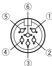
Vista pannello posteriore TS-450S/690S/850S/950SDX
