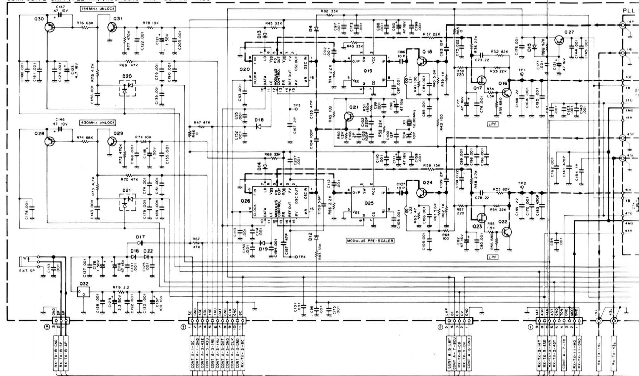
COMPOSITE UNIT (PLL-TX) (X60-3010-XX) -00 TW-4100
