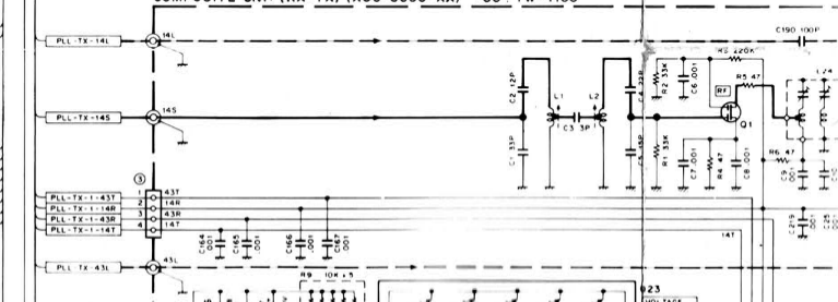
COMPOSITE UNIT (RX-TX) (X60-3000-XX) -00 TW-4100
