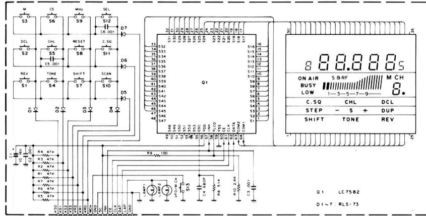
KEYBOARD ASS'Y (W03-2003-05)
