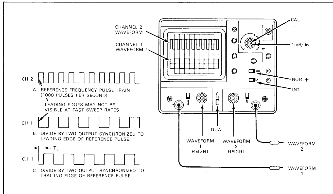
Fig. 4 Waveforms in divide-by-two circuit
