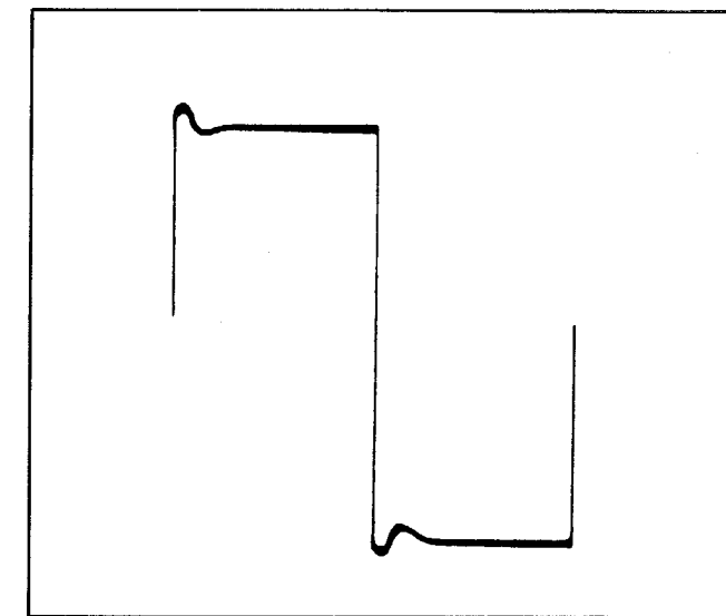
Fig. 33 Effect of high-frequency boost and good damping
