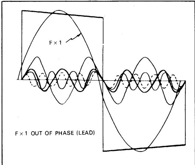
Fig. 29 Tilt resulting from phase shift of fundamental frequency in a leading direction
