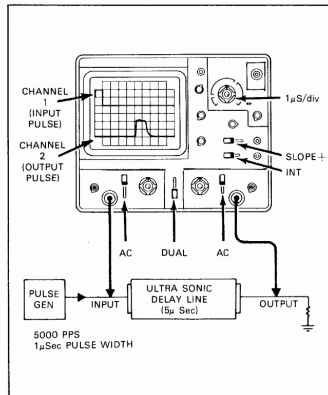
Fig. 8 Delay line measurements
