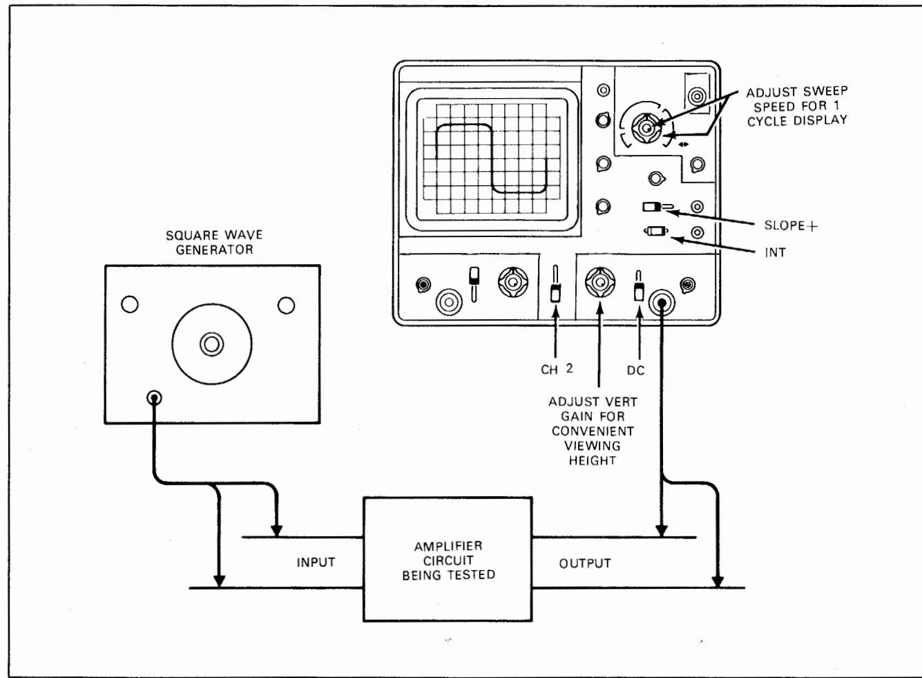
Fig. 23 Equipment set-up for square wave testing of amplifiers
