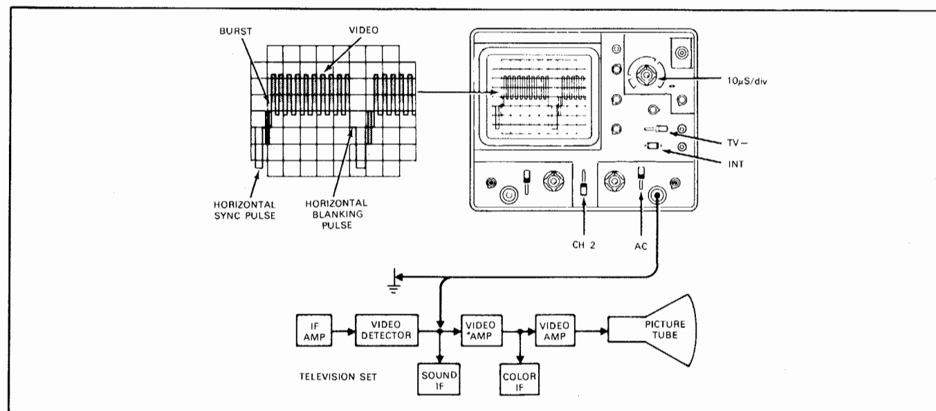
Fig. 14 Set up for viewing horizontal fields of composite video signal
