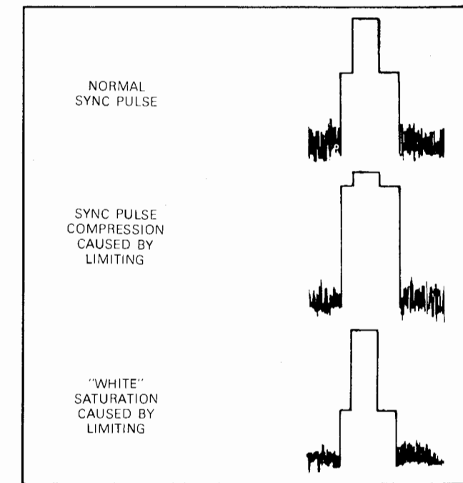
Fig. 17 Sync pulse waveforms
