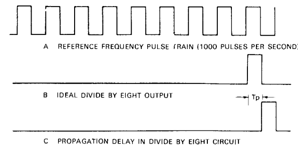
Fig. 3 Waveforms in divide-by-eight circuit
