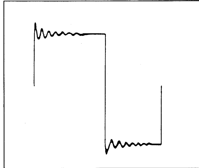
Fig. 32 Effect of high-frequency boost and poor damping
