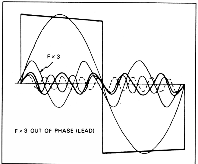
Fig. 38 Square wave tilt resulting from 3rd harmonic phase shift
