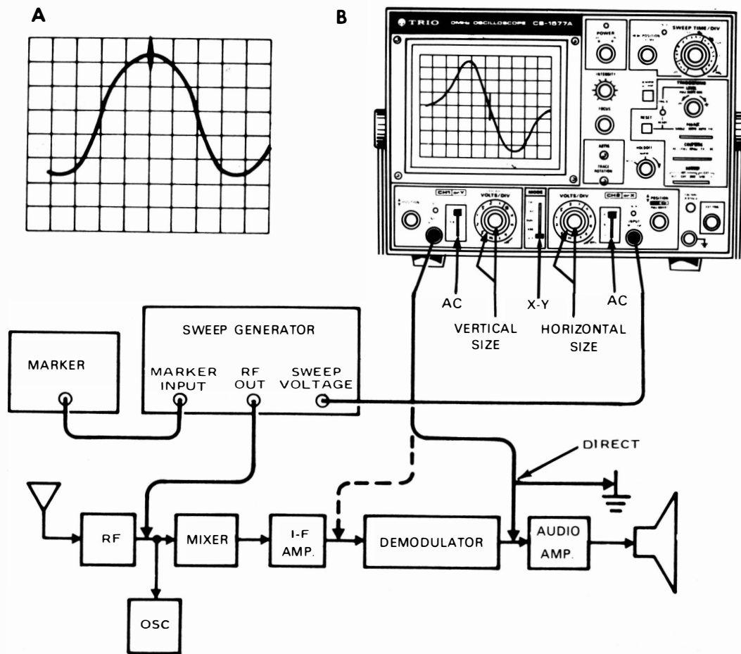
Fig. 28 Typical FM receiver alignment set-up
