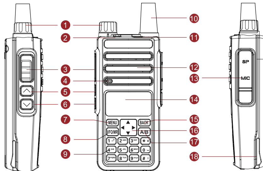
Figure 2.1. Radioddity GA-510, overview
