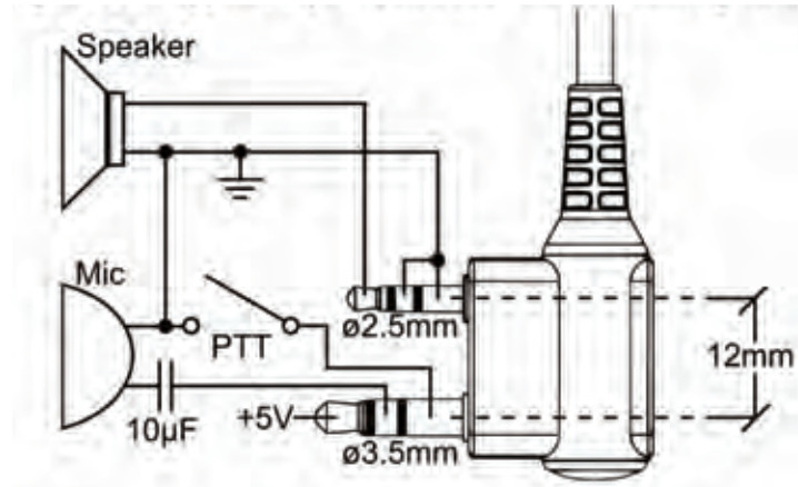
Figure 2.3. Typical 2 pin Kenwood headset configuration.
