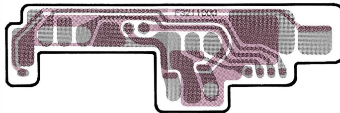
obverse view of "solder" side
