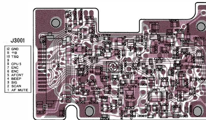
obverse view of "chip-only" side
