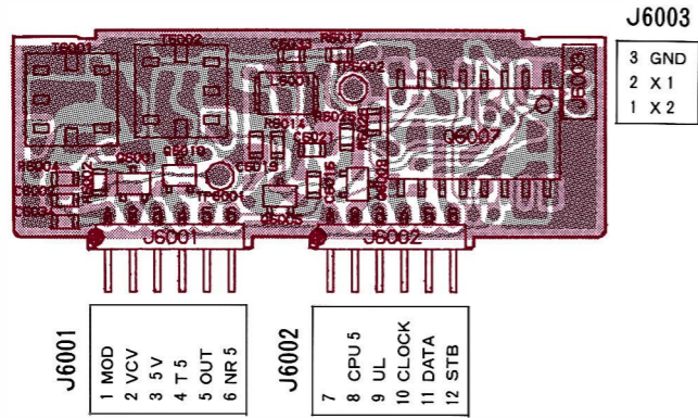
obverse view of "component" side
