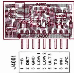
obverse view of "component" side
