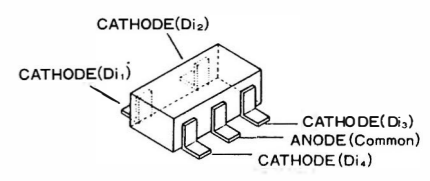
FMP1 (P1) (D2002, 2005)
