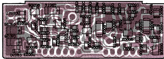
obverse view of "chip-only" side
