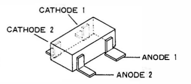
1SS272 (A4) (D2004, 2006)
