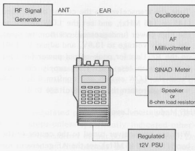
VHF RECEIVER ALIGNMENT SETUP
