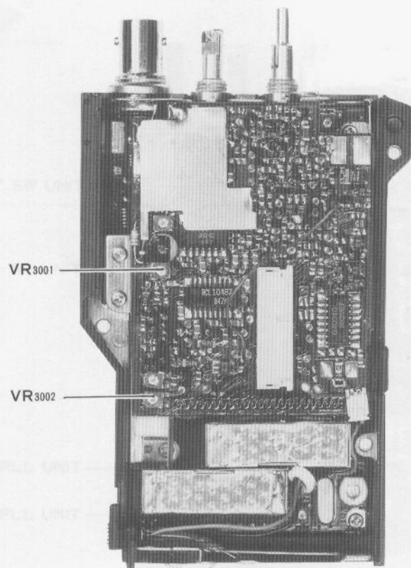
VHF RECEIVER ALIGNMENT POINTS
