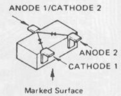
1SS302(C3) (D1013)
