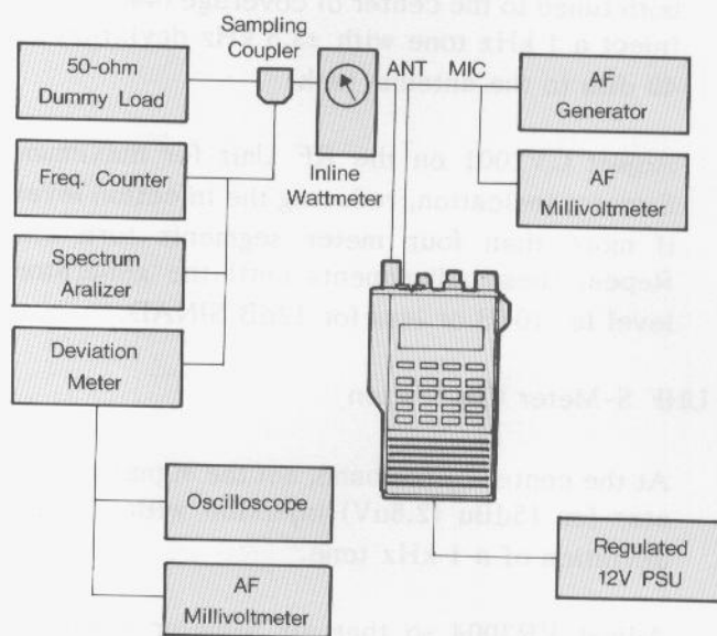
UHF PLL & TRANSMITTER ALIGNMENT SETUP
